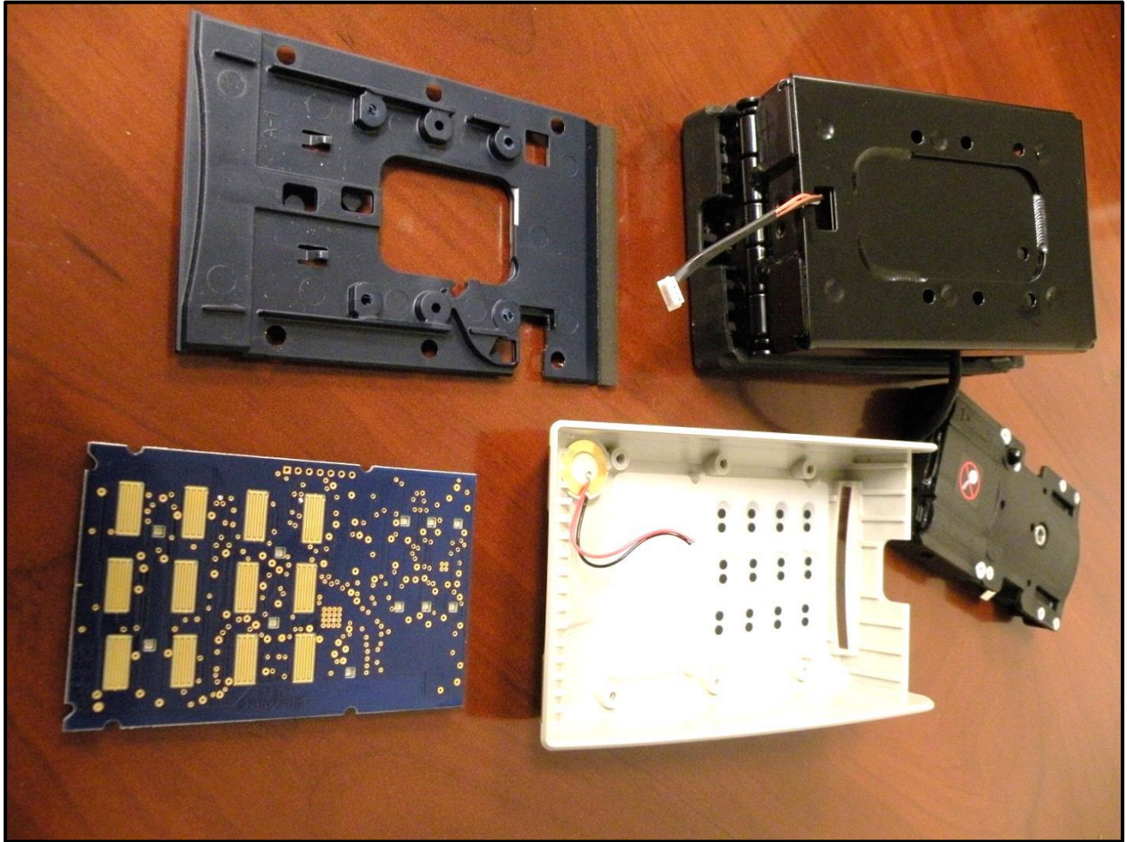
Photograph 13: Board Removed
