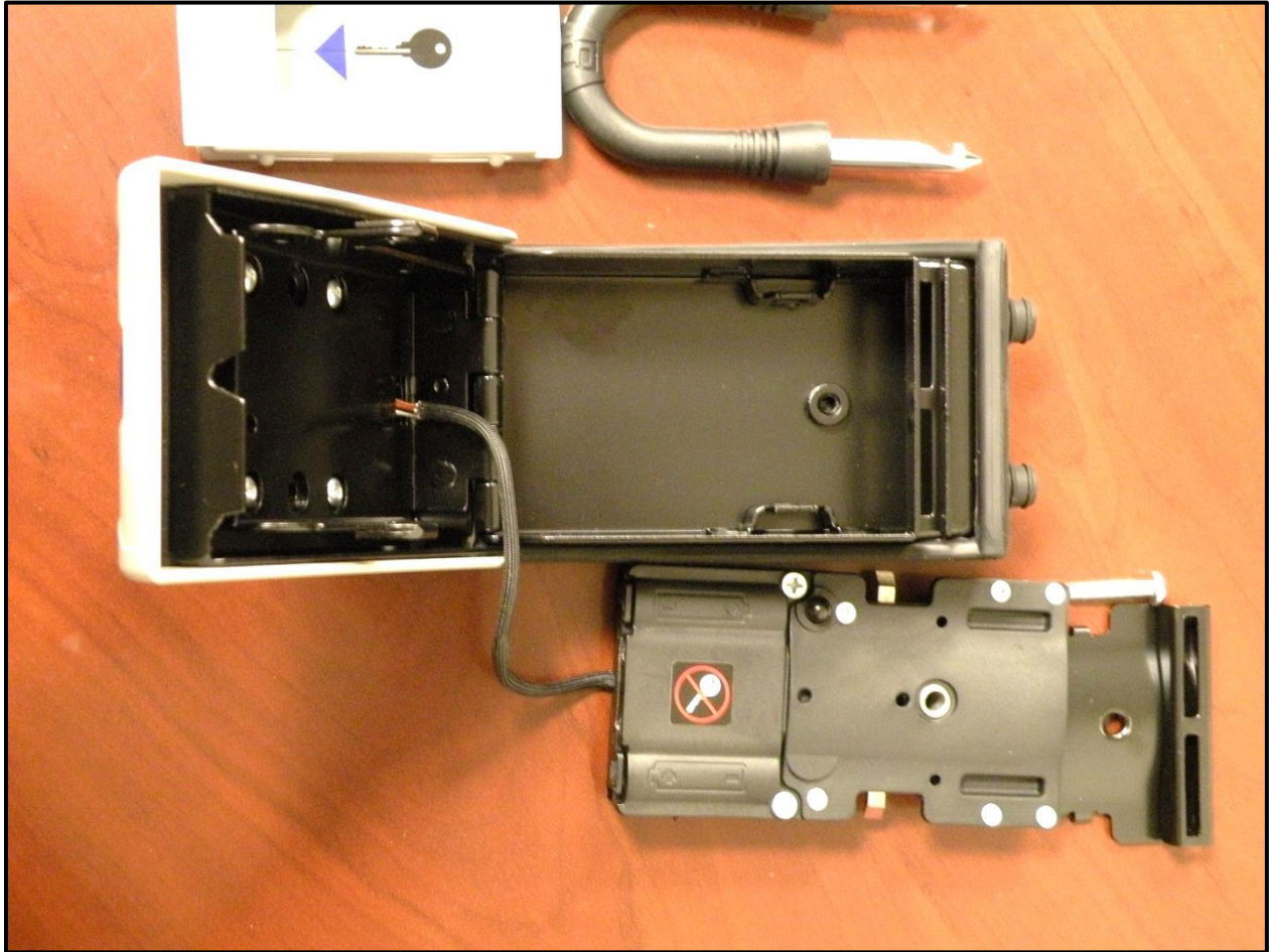
Photograph 9: Front Panel Removed
