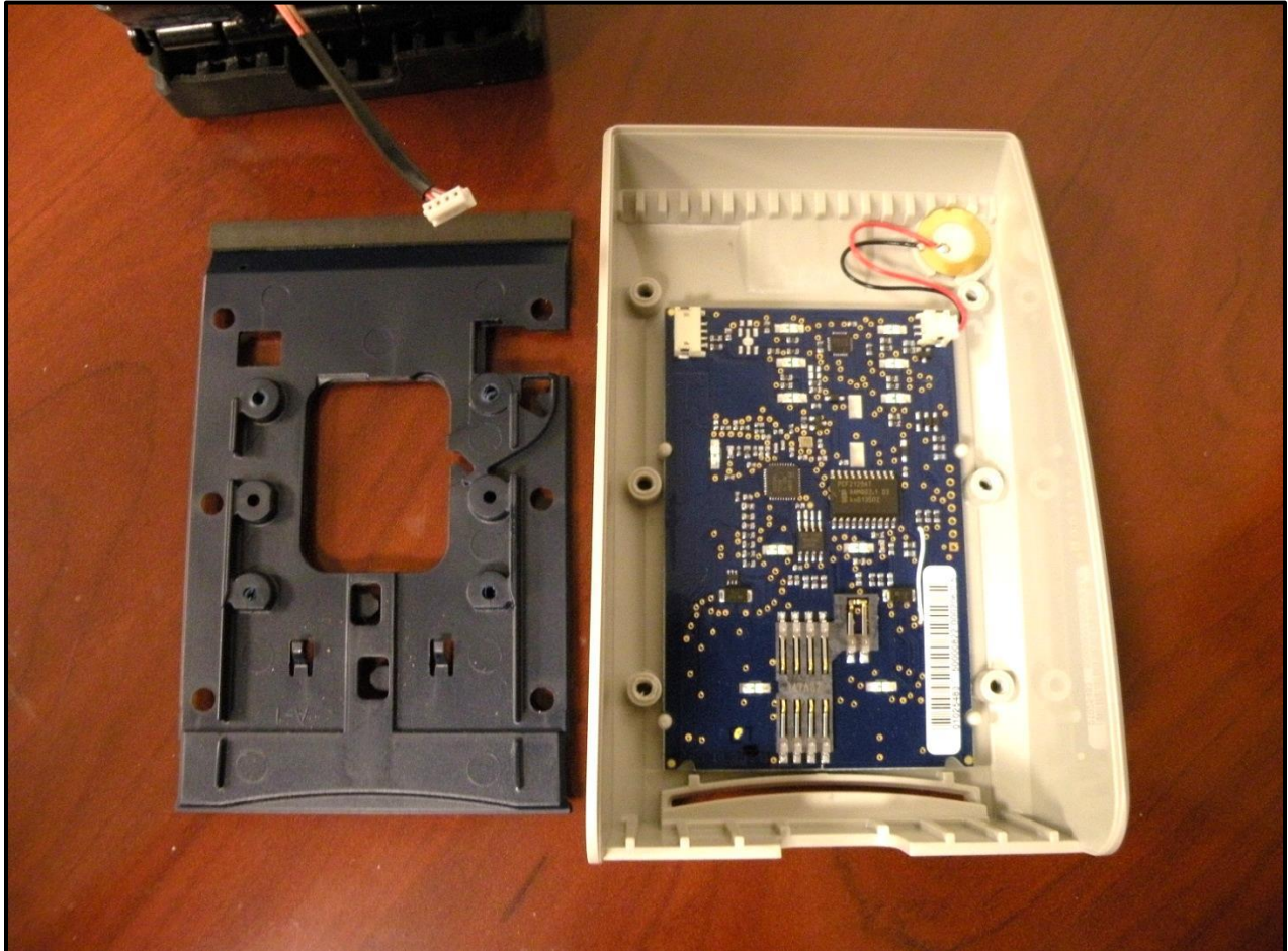
Photograph 11: Front Panel Interior View
