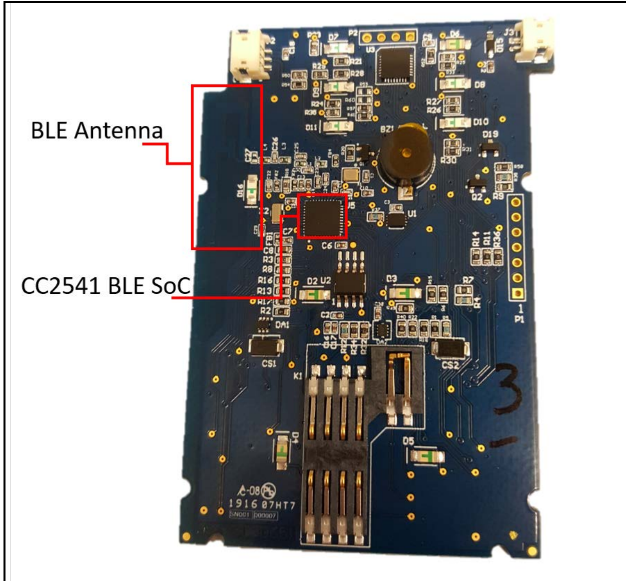
Photograph 12: Main Board – Back
