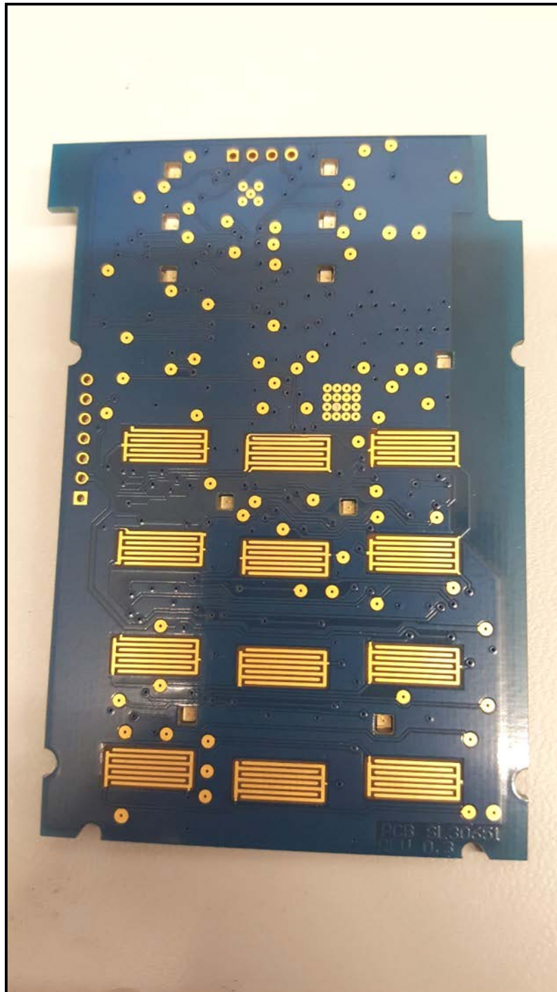
Photograph 11: Main Board – Front
