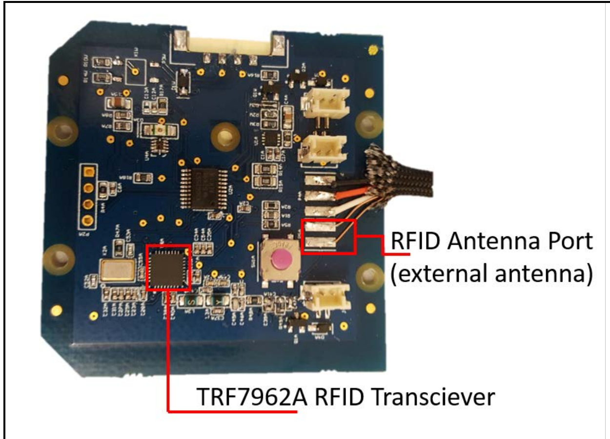
Photograph 13: Vault Board – Front
