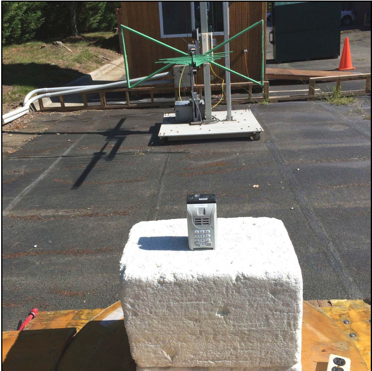
Photograph 5: Radiated Testing – Front View
