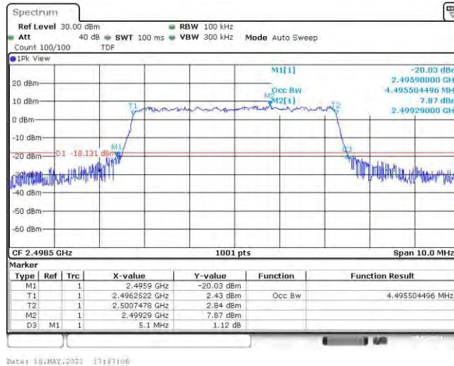
Band41-5MHz-16QAM-40690-25RB#0
