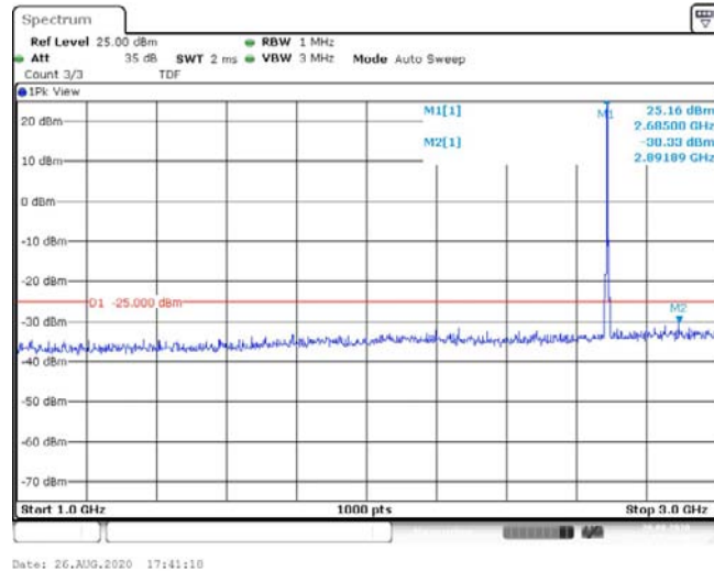
Band41-5MHz-QPSK-41565-1RB#0-Range2:1000~3000MHz--30.33-PASS
