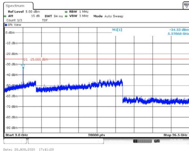
Band41-5MHz-QPSK-41565-1RB#0-Range3:3000~26500MHz--34.53-PASS
