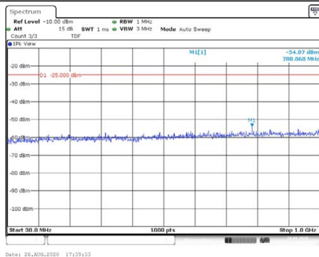
Band41-5MHz-16QAM-39675-1RB#0-Range1:30~1000MHz--54.07-PASS
