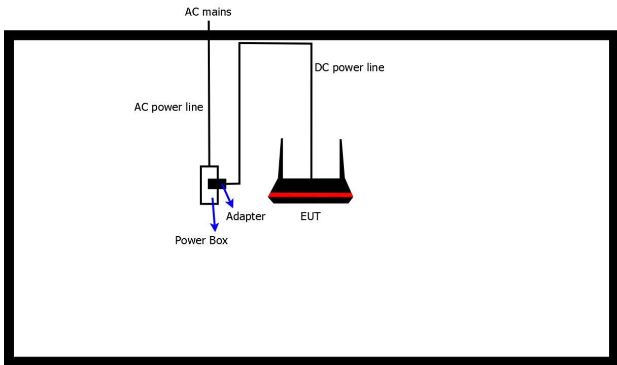
Test Setup Diagram - Radiated Test (Mode 1,2)
