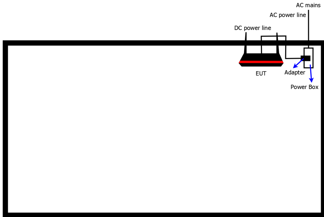
Test Setup Diagram - Radiated Test (Mode 1,2)
