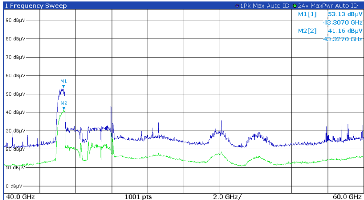
Figure 4.1 Radiated Spurious Emissions 40 – 60 GHz (Horizontal)
