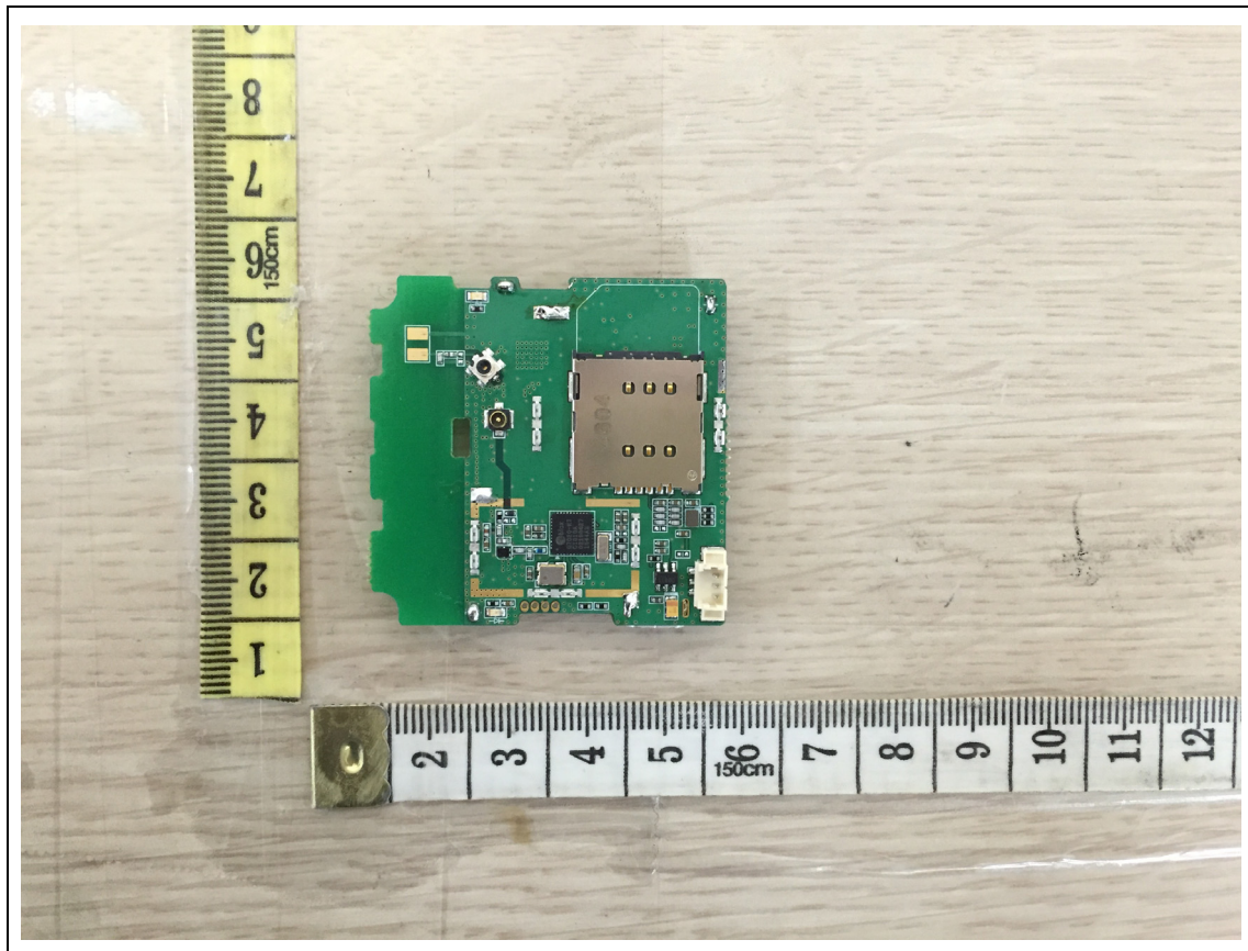
GSM Board 1 Rear
