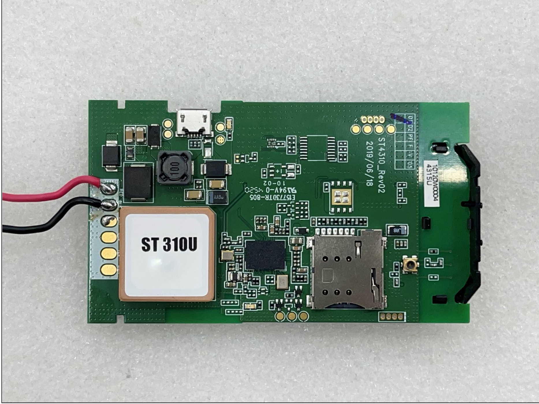
Main Board_Rear
