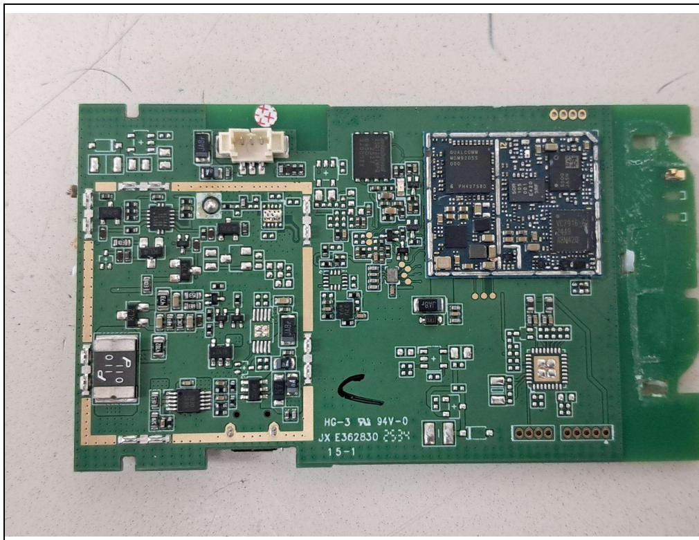
Bottom view of Main PCB(without shield-can)
