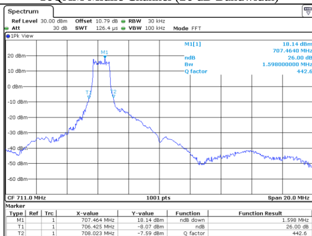
16QAM High Channel (26 dB Bandwidth)
