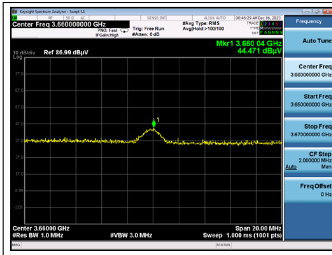
Middle channel Spurious harmonic (Peak)
