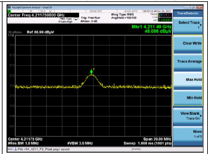
Low channel Spurious harmonic (Peak)
