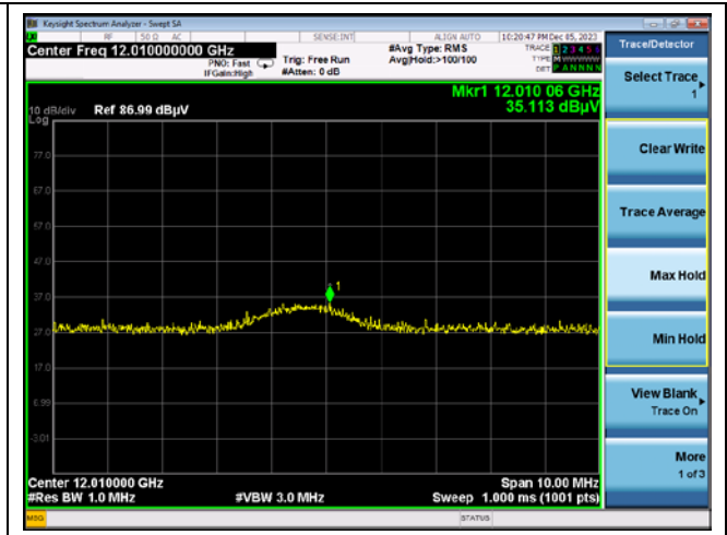
Low channel 5 th harmonic (Peak)
