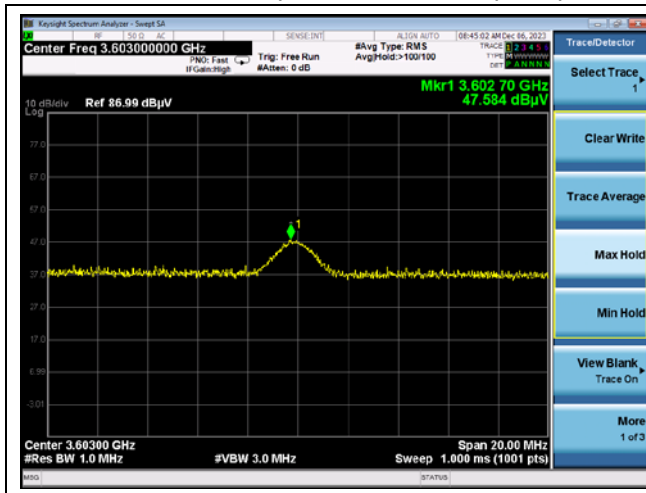
Low channel Spurious harmonic (Peak)
