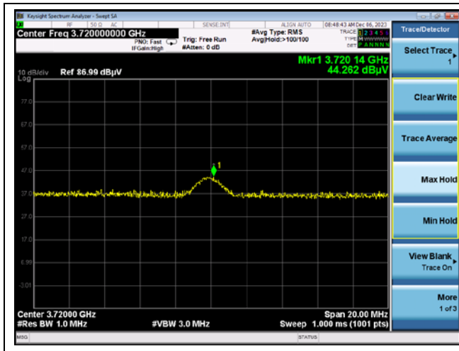
High channel Spurious harmonic (Peak)
