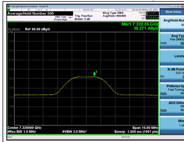
Middle channel 3 rd Harmonic (Average)
