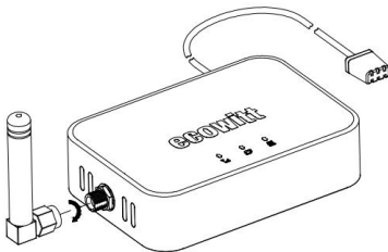
Figure 1 Install Antenna
