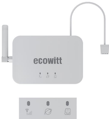
Figure 5 LED Indicators
