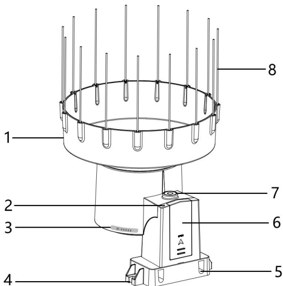
Figure 8 Sensor Assembly Components
