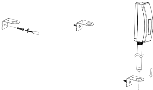
Figure 3-1: Sensor mounting
