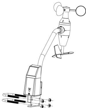
Figure 2: U-Bolt installation
