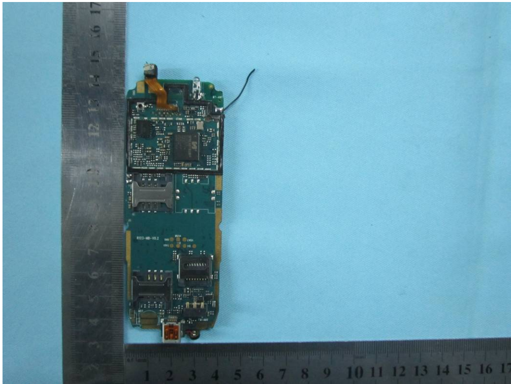
Mainborad Without Shielding - Front View (I129)
