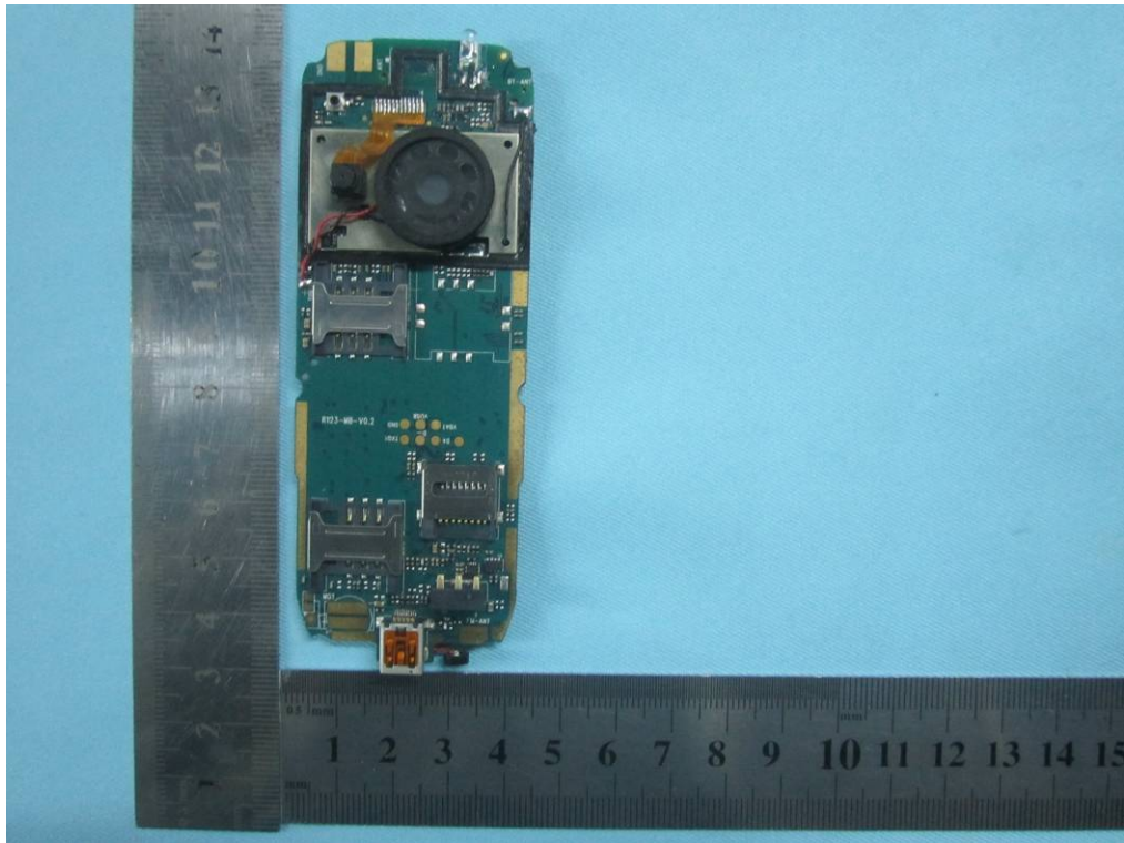
Mainborad With Shielding - Front View (I129)
