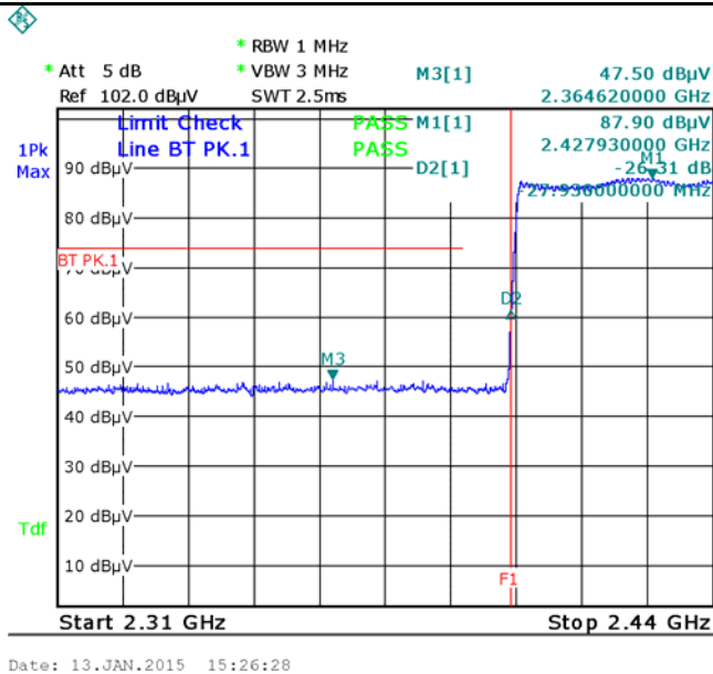
8DPSK-Hopping Left-PK
