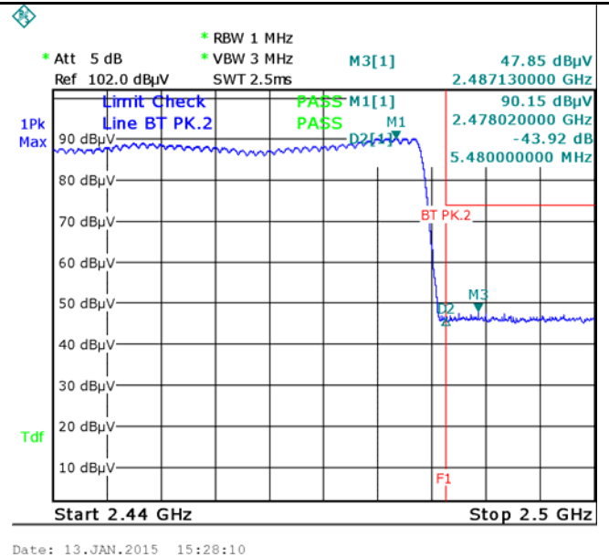
8DPSK-Hopping Right-PK
