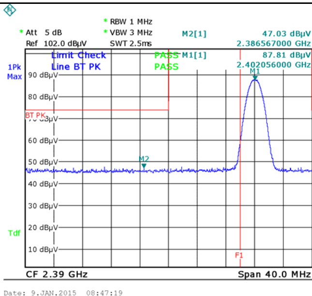
8DPSK-Left Side-PK
