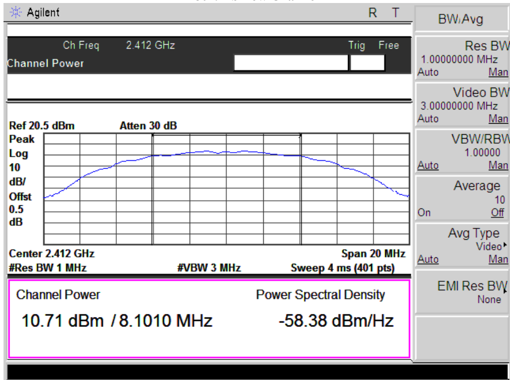
802.11b Low Channel
