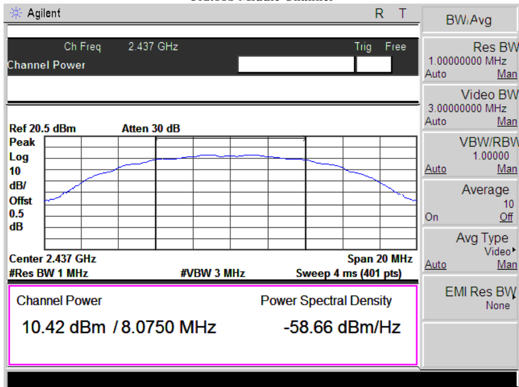
802.11b Middle Channel
