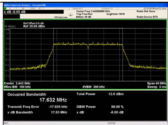
802.11n20 6dB Bandwidth - Mid CH 2442
