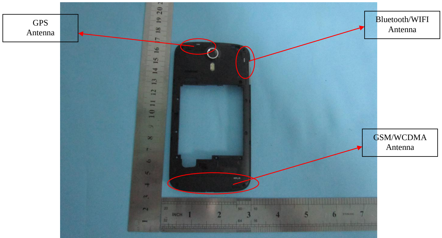
Antenna View
