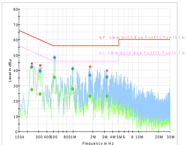
Fig.63 AC Powerline Conducted Emission
