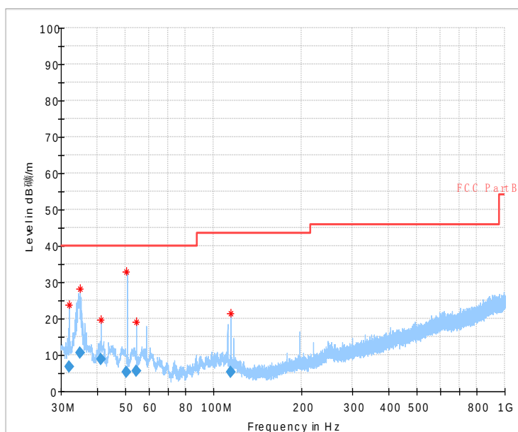
Fig.59 Radiated Spurious Emission (802.11g,Ch11,30MHz~1GHz)
