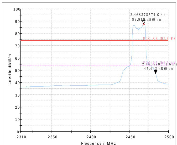
Fig.58 Radiated emission (Power): 802.11g, high channel
