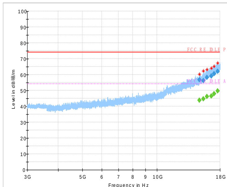
Fig.61 Radiated Spurious Emission (802.11g,Ch11,3GHz~18GHz)
