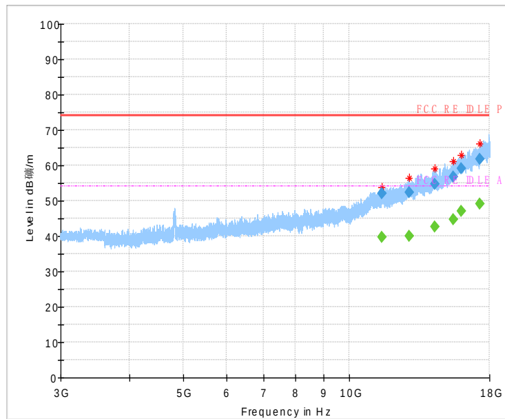
Fig.57 Radiated Spurious Emission (802.11 n-20MHz,Ch1,3GHz~18GHz)
