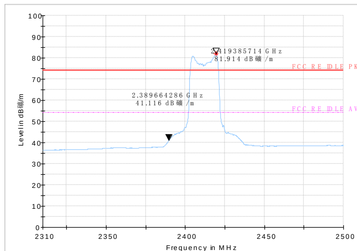
Fig.53 Radiated emission (Power): 802.11n, low channel
