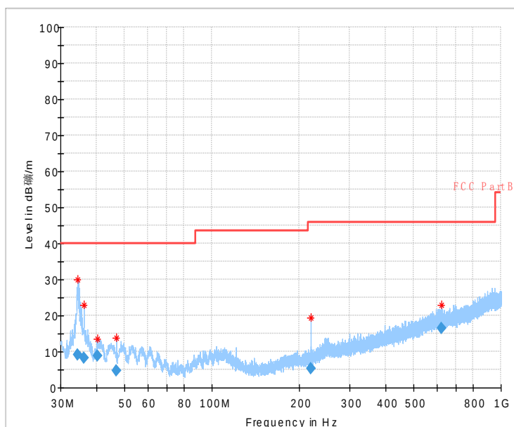
Fig.45 Radiated Spurious Emission (802.11b,Ch1,30MHz~1GHz)
