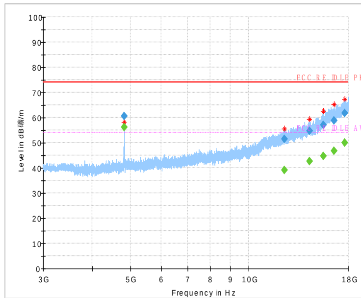
Fig.47 Radiated Spurious Emission (802.11b,Ch1,3GHz~18GHz)
