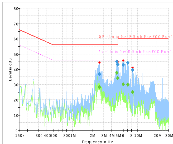
Fig.62 AC Powerline Conducted Emission
