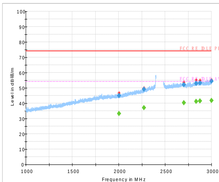
Fig.46 Radiated Spurious Emission (802.11b,Ch1,1GHz~3GHz)
