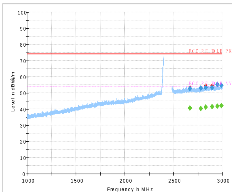
Fig.51 Radiated Spurious Emission (802.11g,Ch1,1GHz~3GHz)
