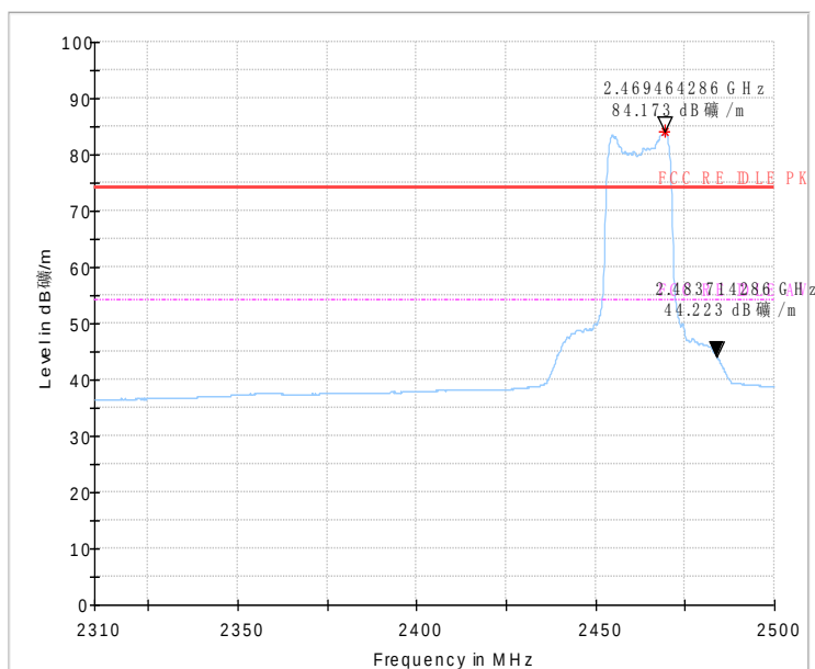
Fig.54 Radiated emission (Power): 802.11n, high channel
