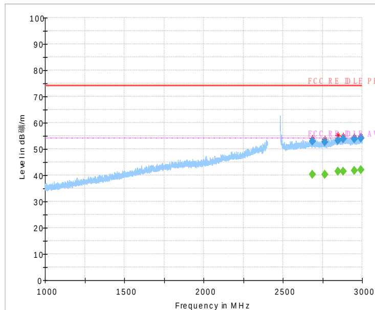
Fig.60 Radiated Spurious Emission (802.11g,Ch11,1GHz~3GHz)
