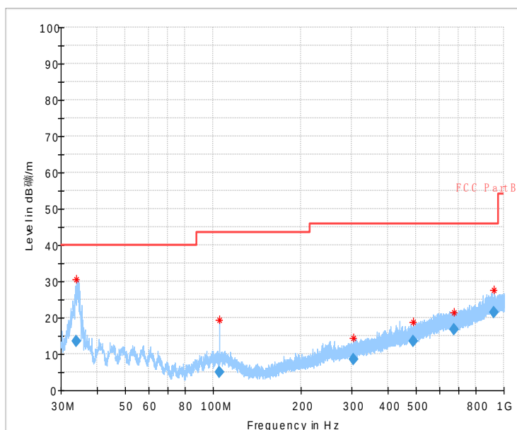
Fig.55 Radiated Spurious Emission (802.11 n-20MHz,Ch1,30MHz~1GHz)
