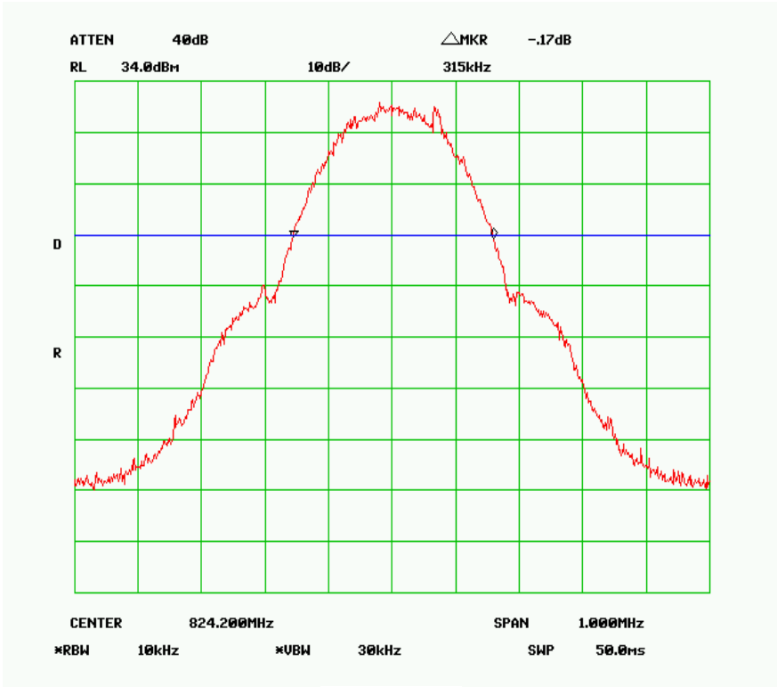
850-26dB-L
