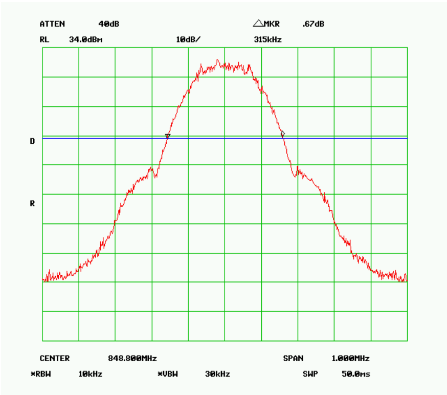
850-26dB-H
