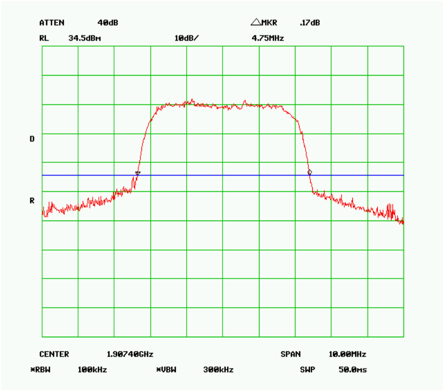
W1900-26dB-H
