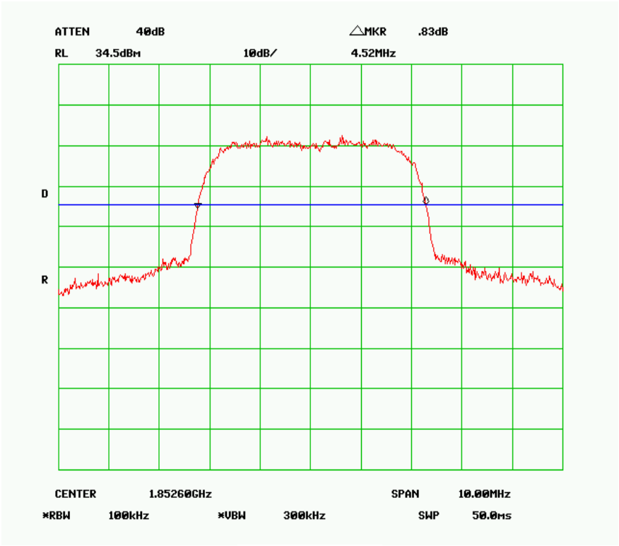
W1900-26dB-L
