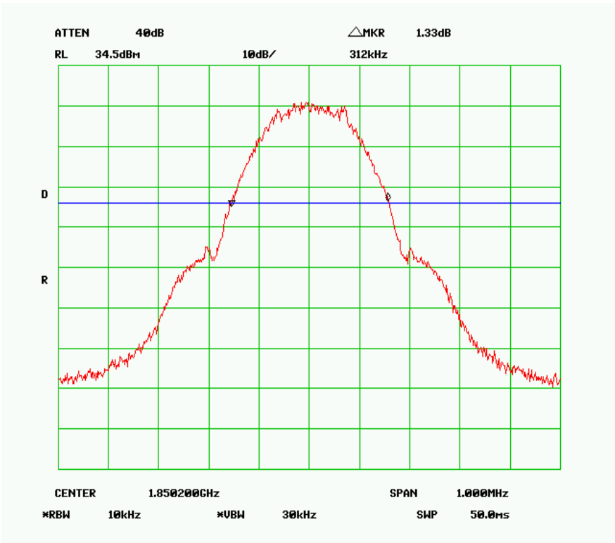
1900-26dB-L
