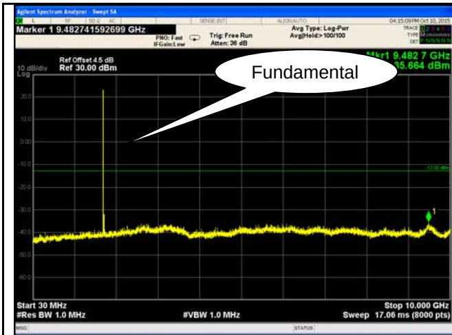
LTE Band 4 - Low Channel-1
