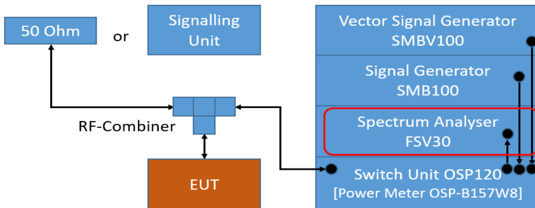
TS8997; Power Spectral Density
