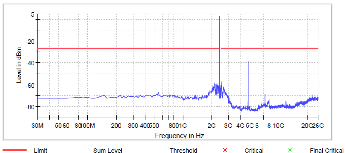
BT LE 1 Mbps Ch 00 Spurious
