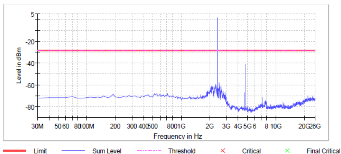
BT LE 2 Mbps Ch 00 Spurious
