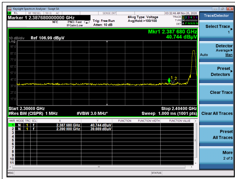
(AVERAGE, Channel 0)
