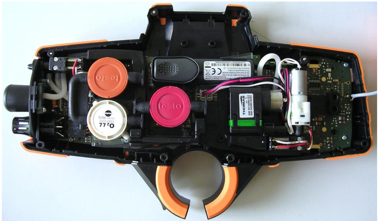
t330i, lower shell, view inside
