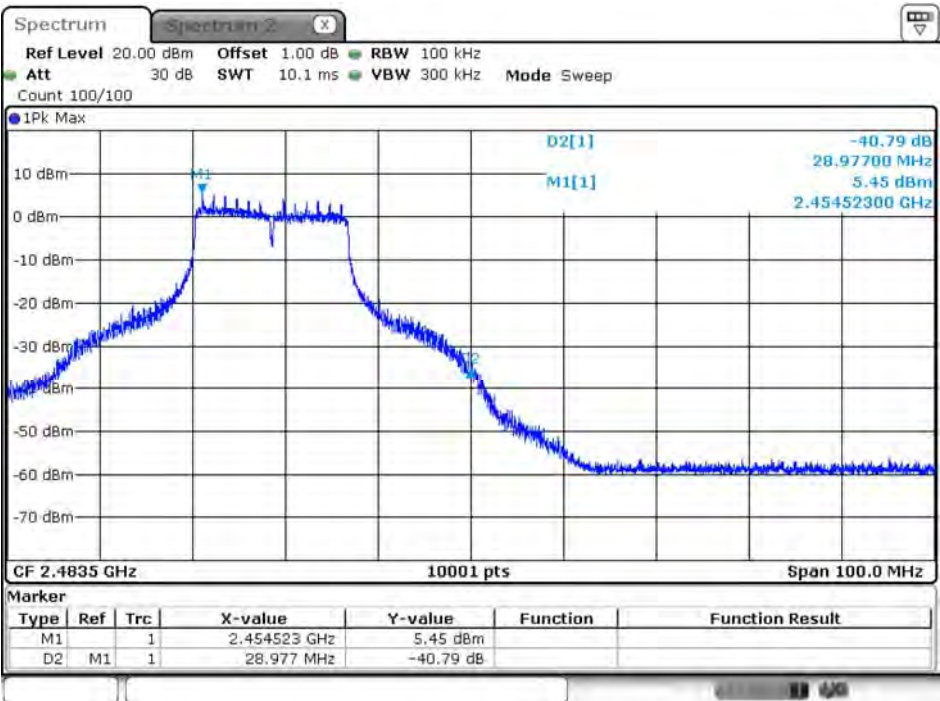
Channel 11 (2462MHz)
