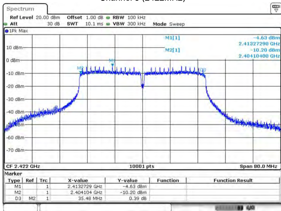
Channel 3 (2422MHz)
