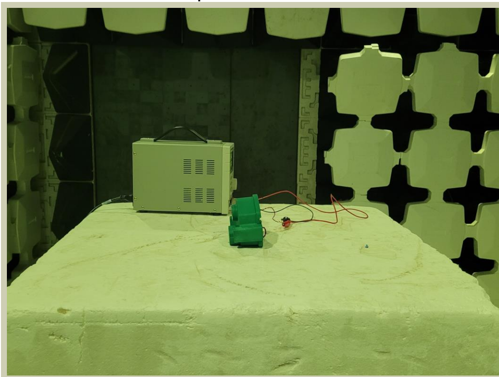
Radiated Spurious – Above 1 GHz
