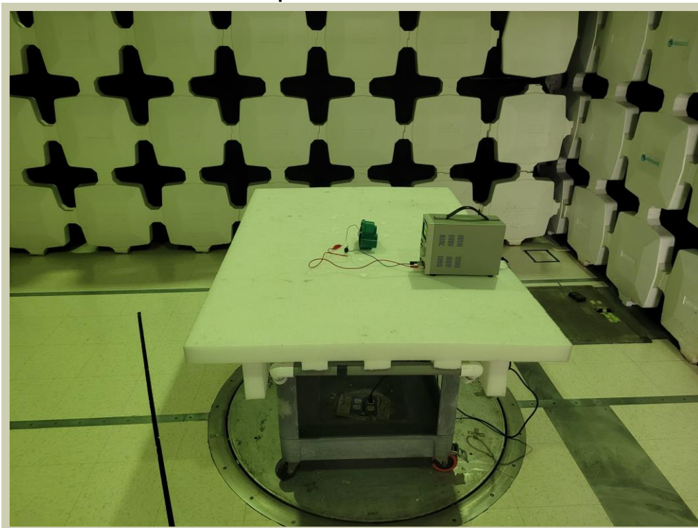
Radiated Spurious – Below 1 GHz
