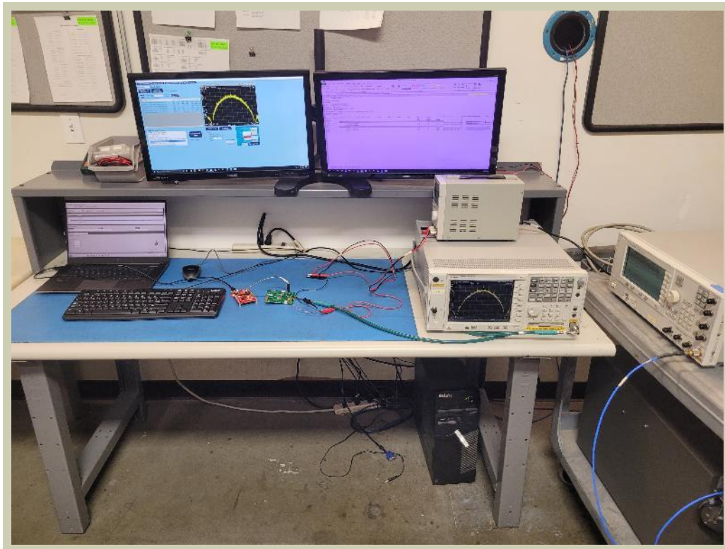
Direct Connect
