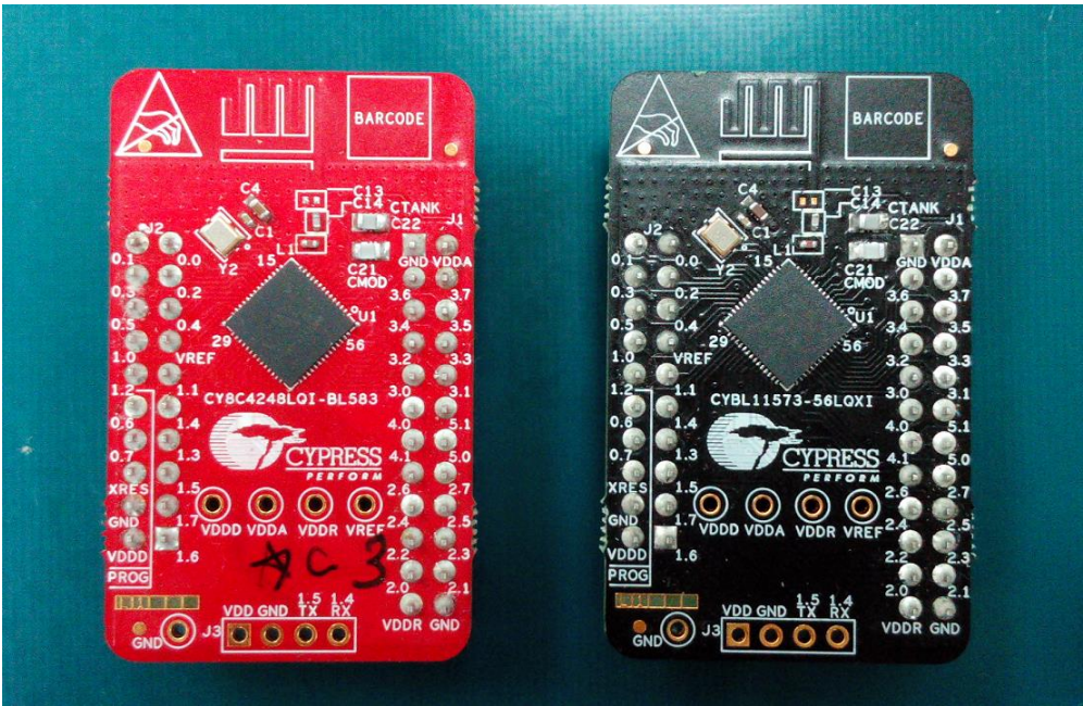
CY8CKIT-143A (left) TOP VS CY5676A (right) TOP
