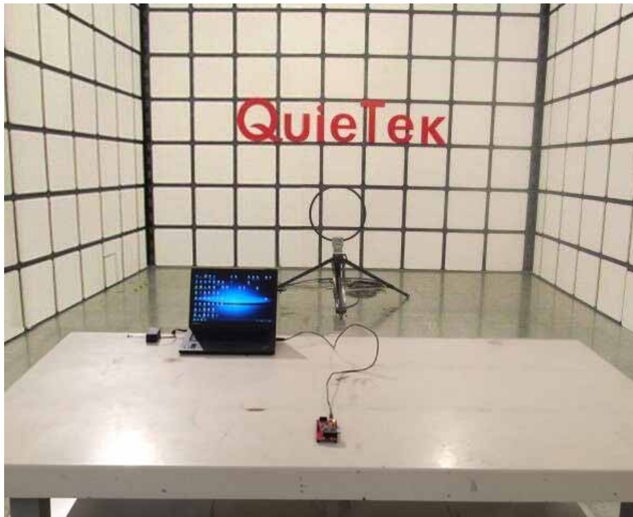
Description: Radiated Emission Test Setup for Below 30MHz
