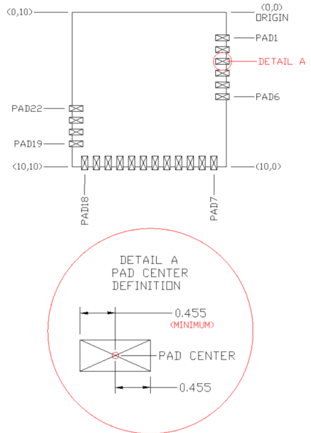
Figure 6. Solder Pad Reference Location
