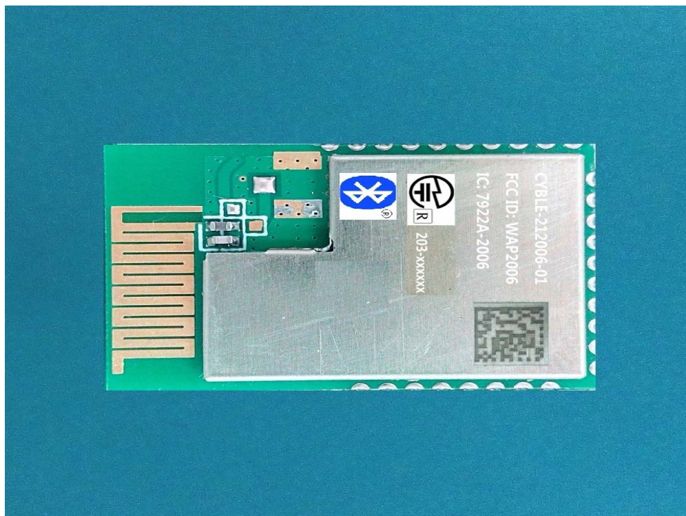
(4) EUT Photo CYBLE-212006-01
