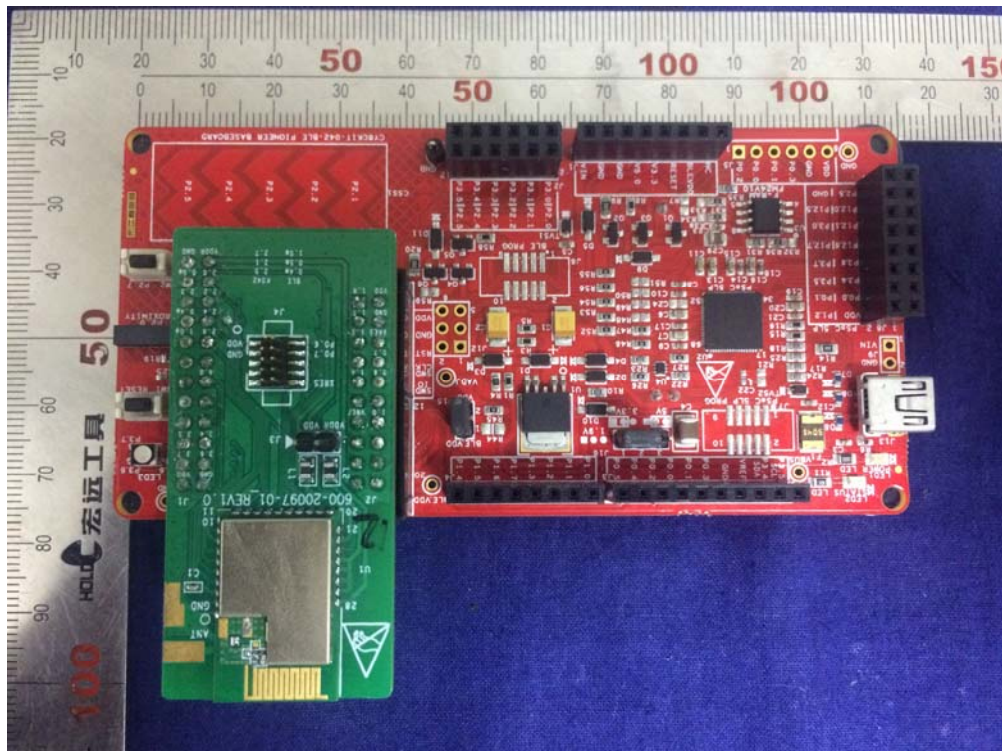
(3) EUT Photo CYBLE-212006-01
