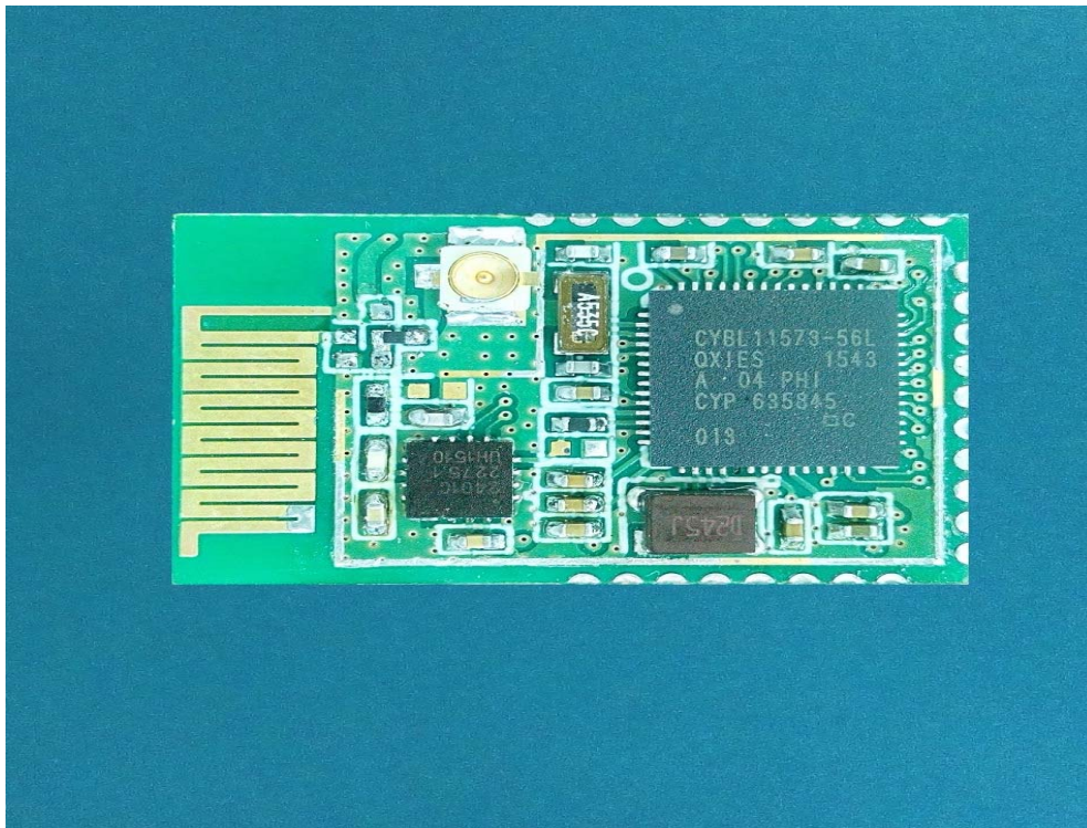
(11) EUT Photo CYBLE-202007-01
