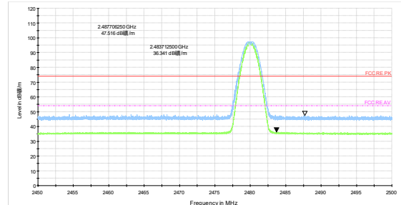
Bluetooth LE (1M) Channel 39 Peak+Average
