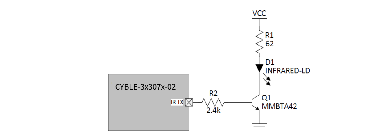
Figure 11 Infrared TX
