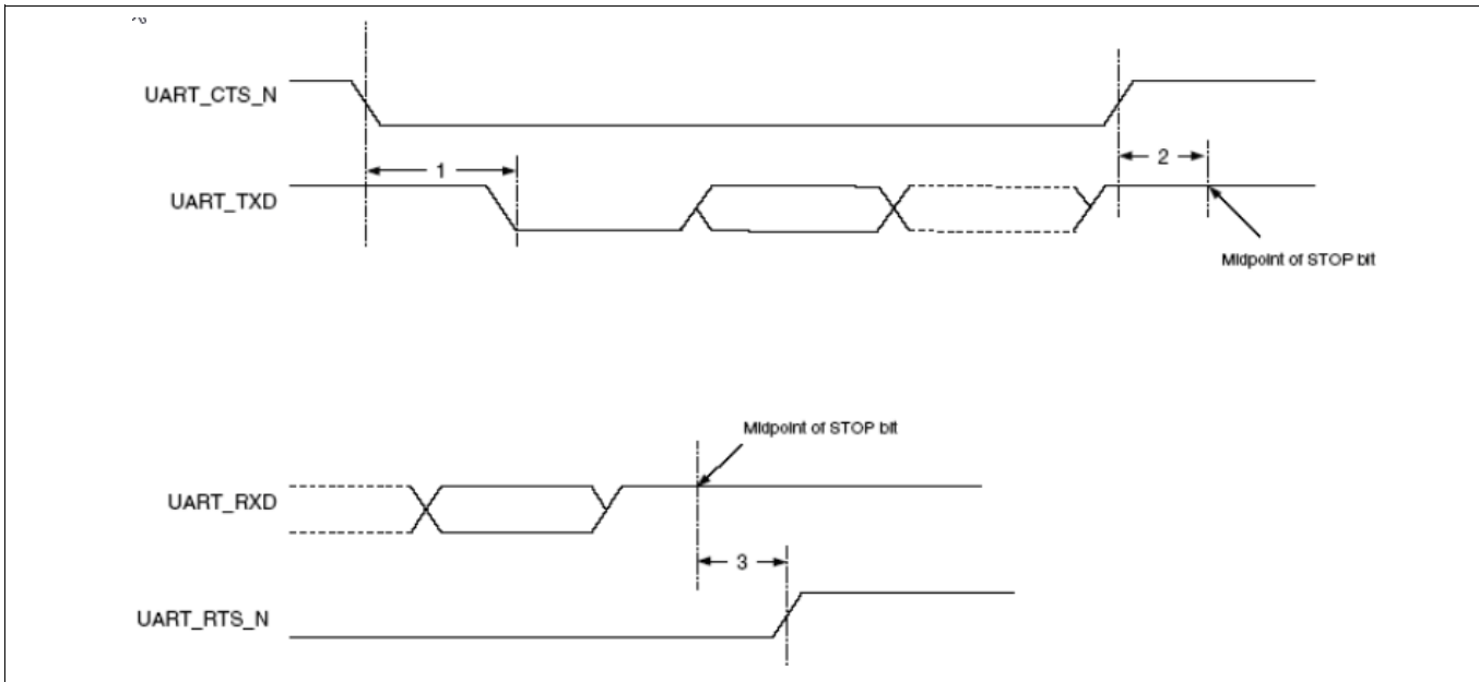
Figure 13 UART timing
