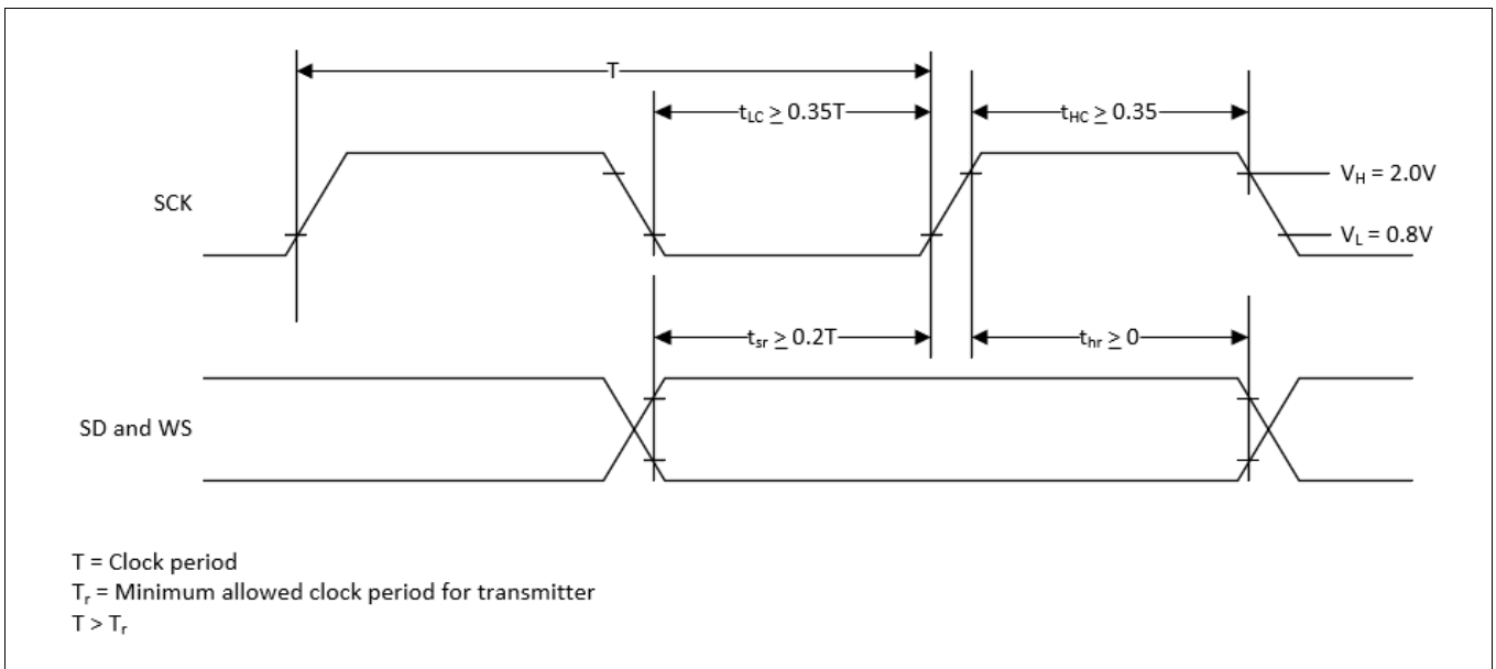
Figure 18 I²S receiver timing
