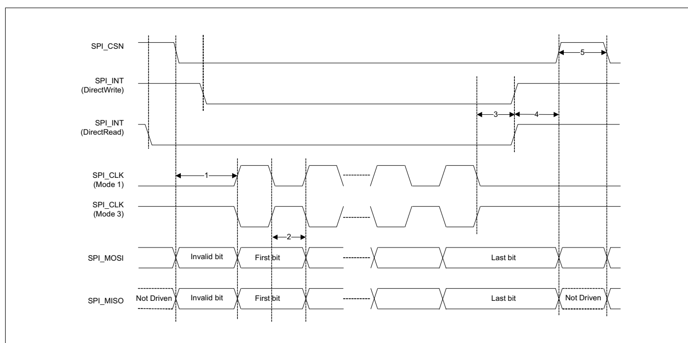
Figure 15 SPI timing – mode 1 and 3
