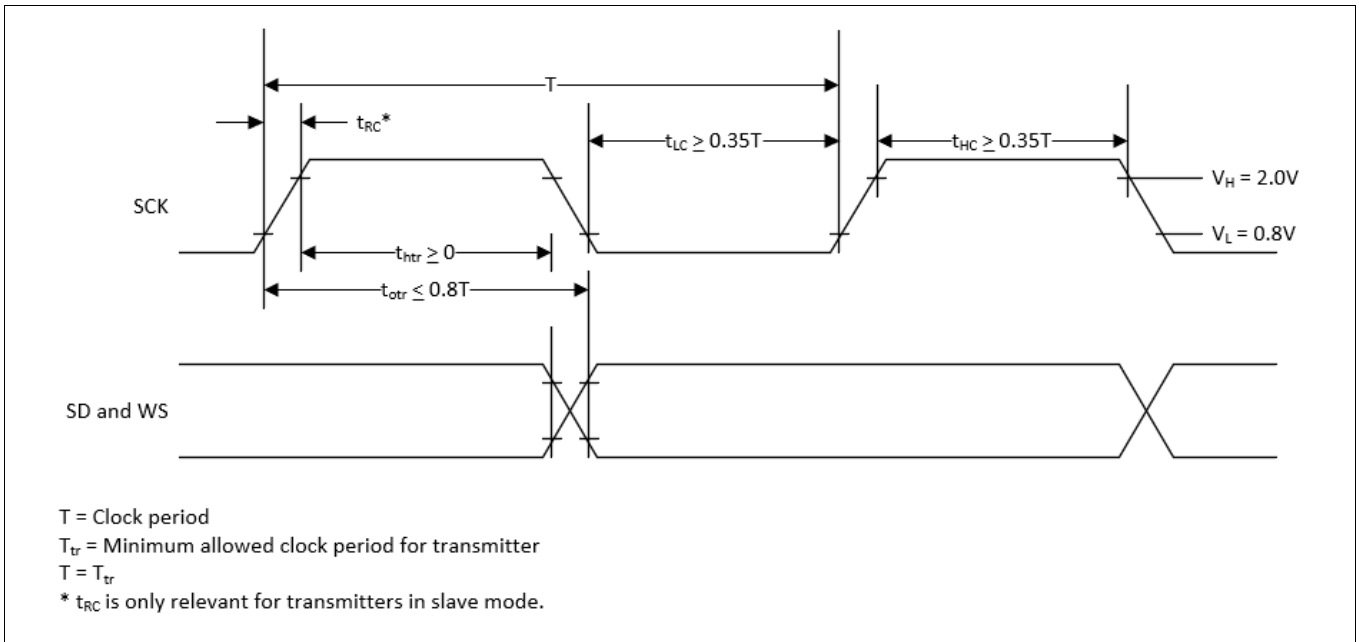
Figure 17 I²S transmitter timing
