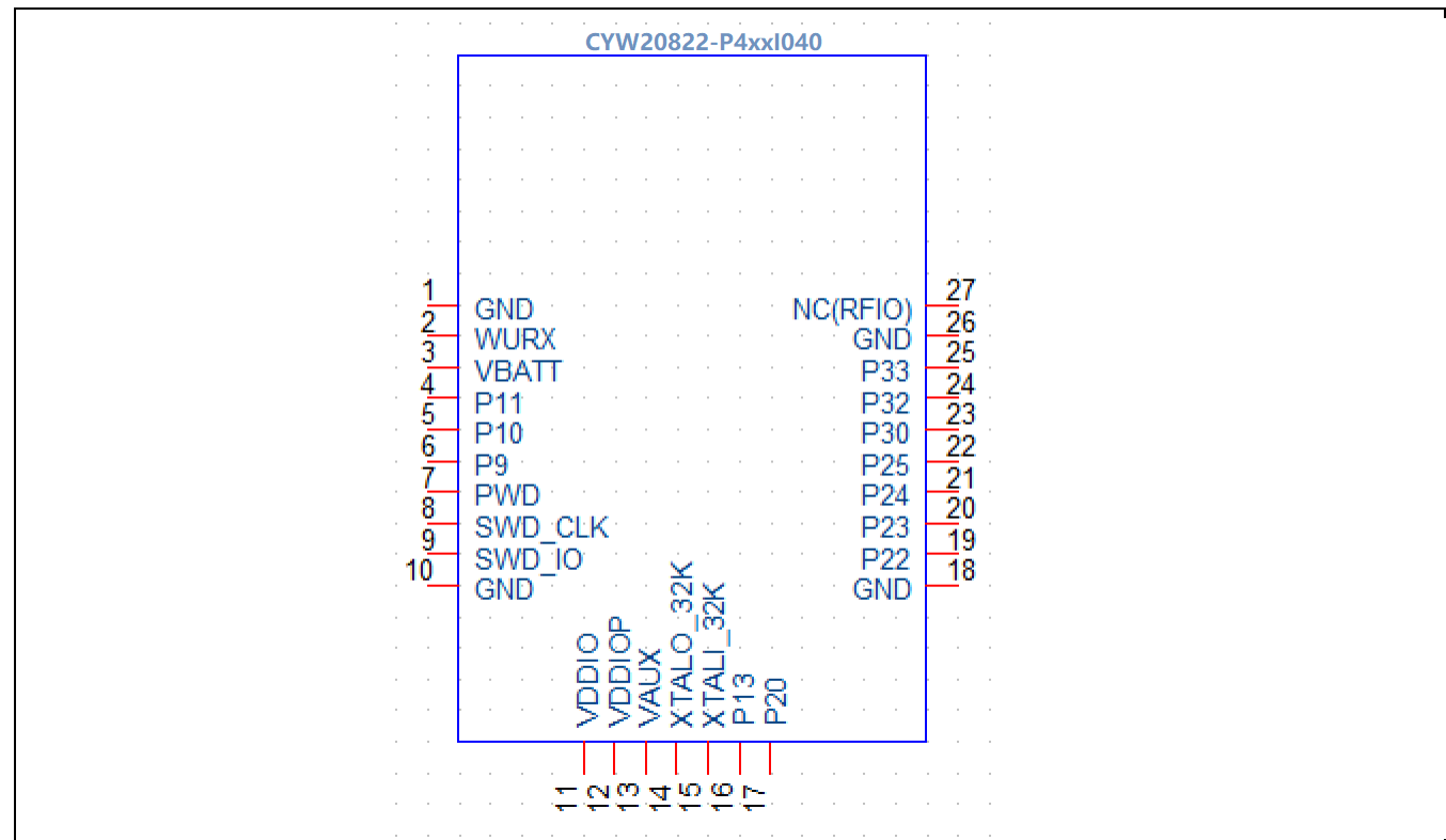
Figure 11 Module pin definition
