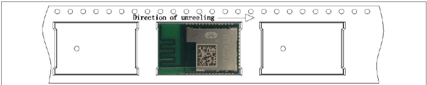
Figure 17 Component orientation in tape and unreeling direction
