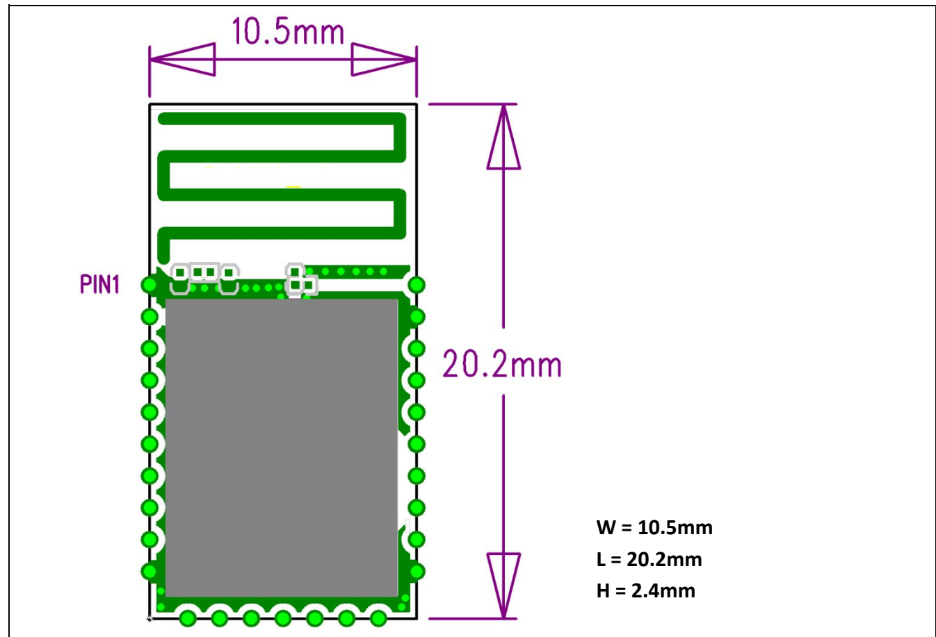
Figure 12 CYW20822-P4XXI040 module with antenna dimensions
