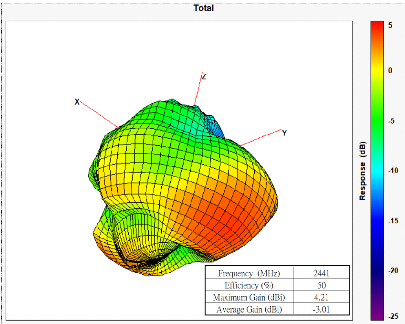
Figure 14 CYW20822-P4XXI040 PCB antenna radiation pattern and characteristics
