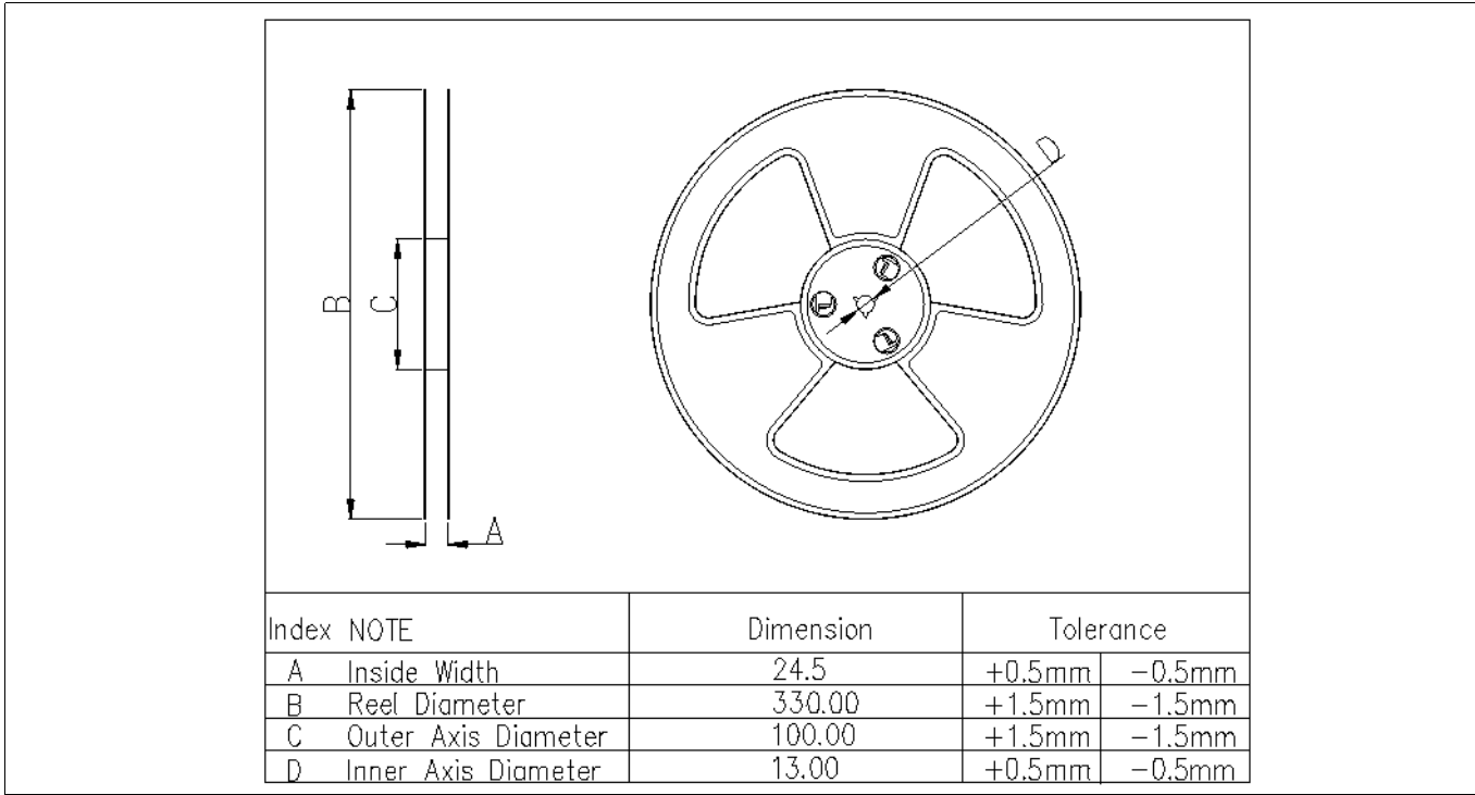
Figure 18 Reel dimensions
