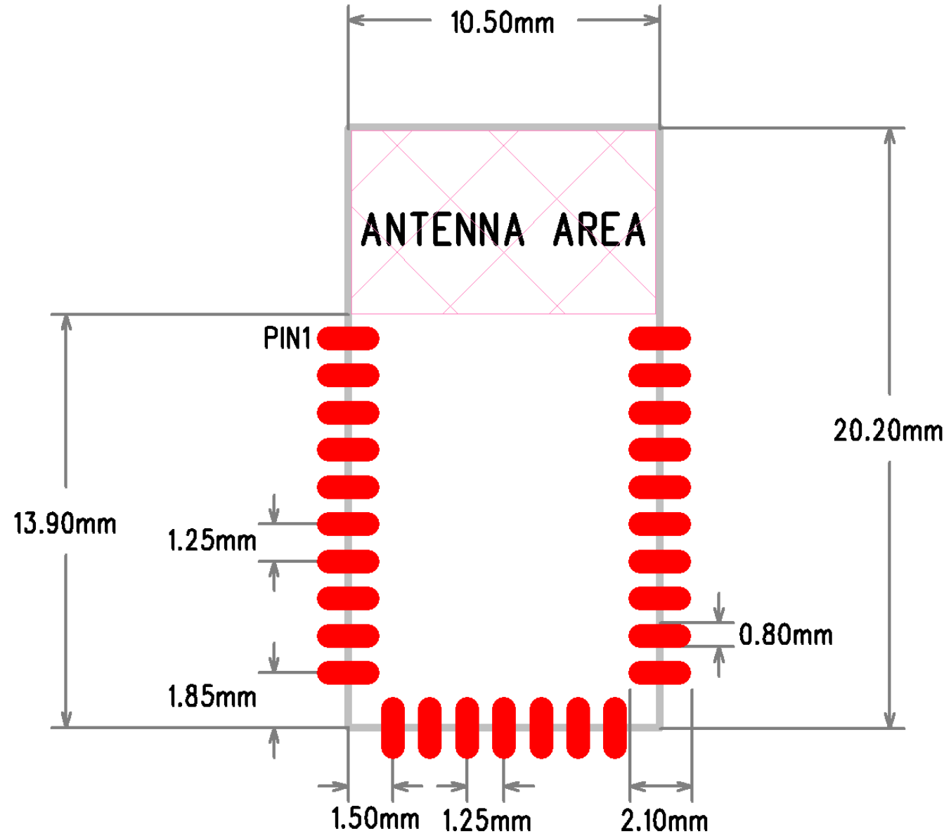
Figure 13 CYW20822-P4XXI040 module - Recommended PCB footprint
