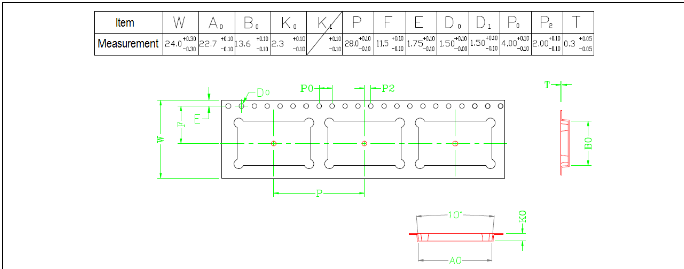
Figure 16 CYW20822-P4xxI040 tape dimensions
