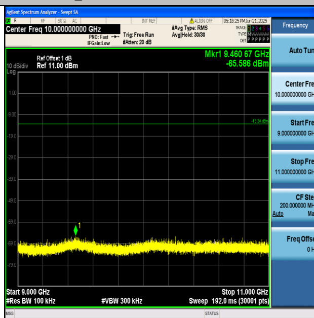
BLE_125K-Ant1-2480-9000~11000-PASS
