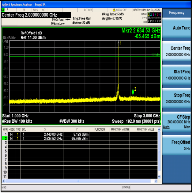
BLE_500K-Ant1-2440-1000~3000-PASS
