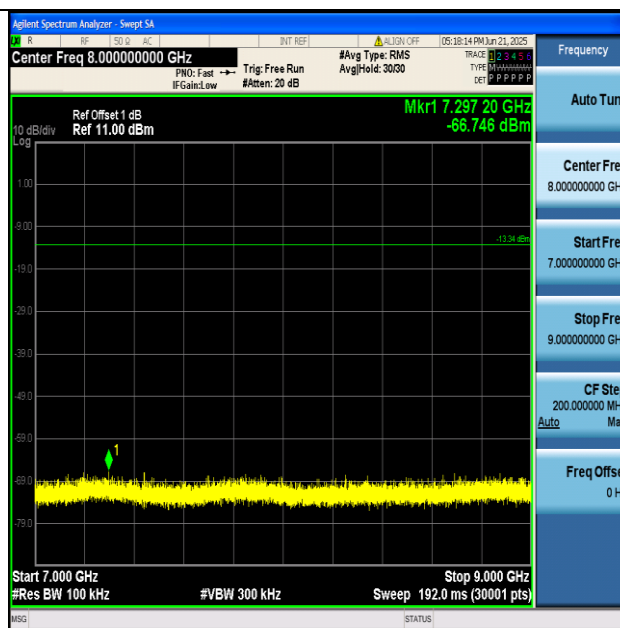
BLE_125K-Ant1-2480-7000~9000-PASS
