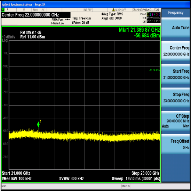
BLE_125K-Ant1-2480-21000~23000-PASS
