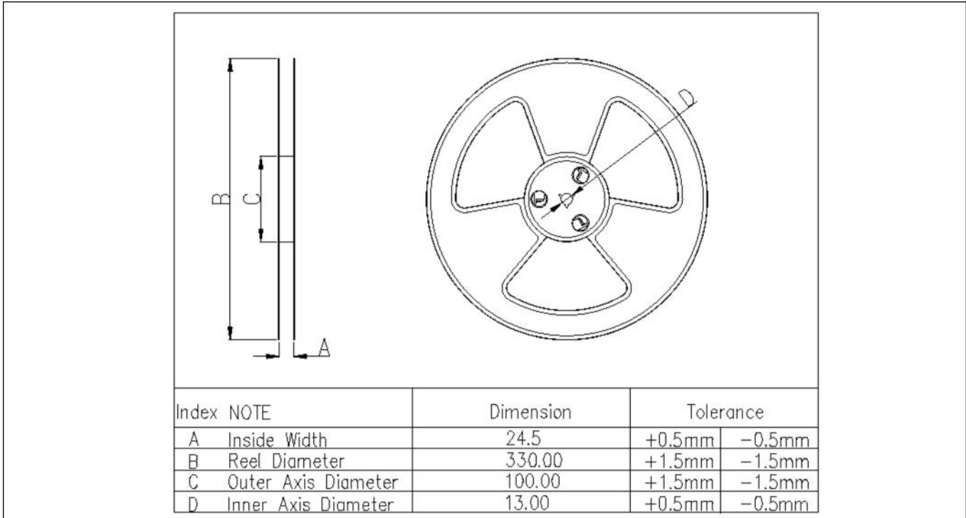
Figure 10 Reel dimensions
