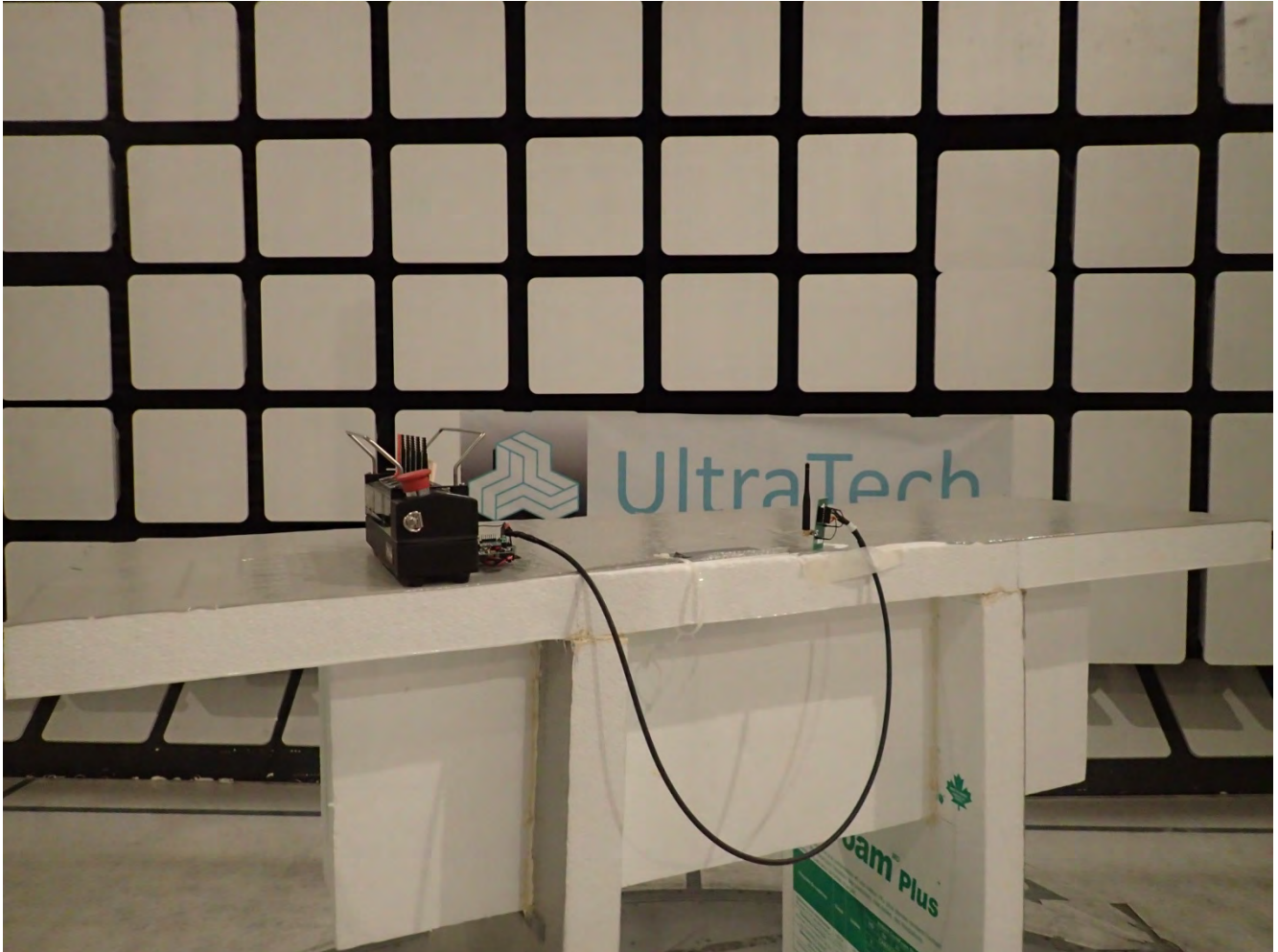
Radiated Emissions @ 3 m EUT with ANT-916-CW-RCL Antenna, Orthogonal Position 3
