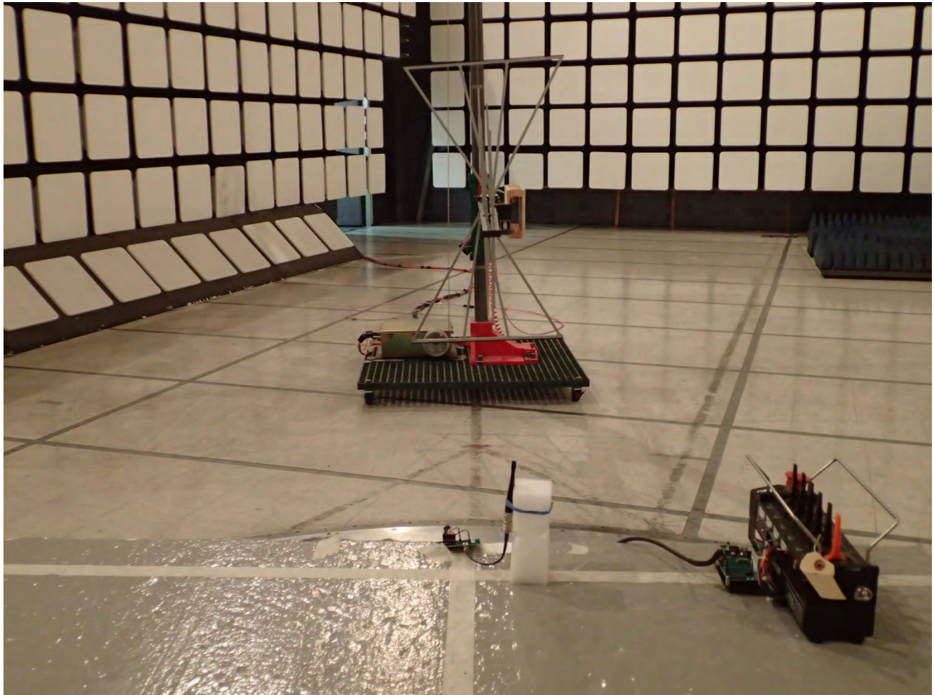
Radiated Emissions @ 3 m EUT with Laird EXC902BNX Antenna, Orthogonal Position 1
