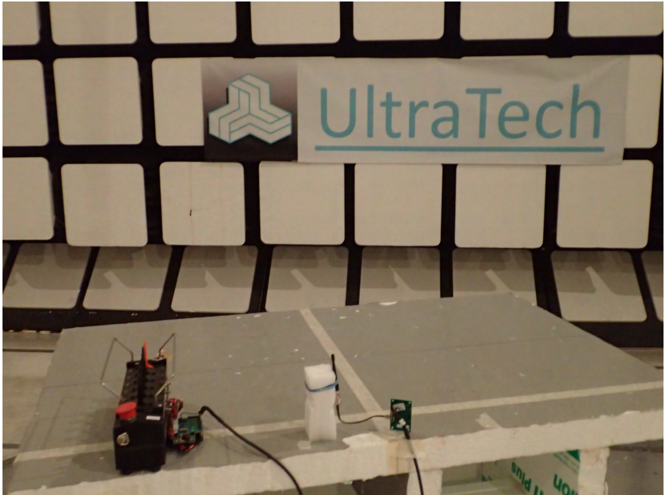
Radiated Emissions @ 3 m EUT with Laird EXC902BNX Antenna, Orthogonal Position 3
