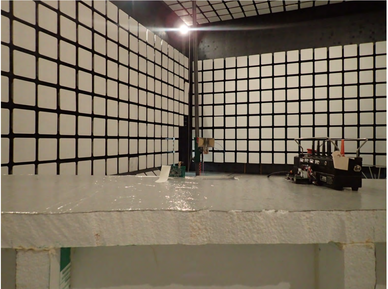
Radiated Emissions @ 3 m EUT with ANT-916-CW-RCL Antenna, Orthogonal Position 2
