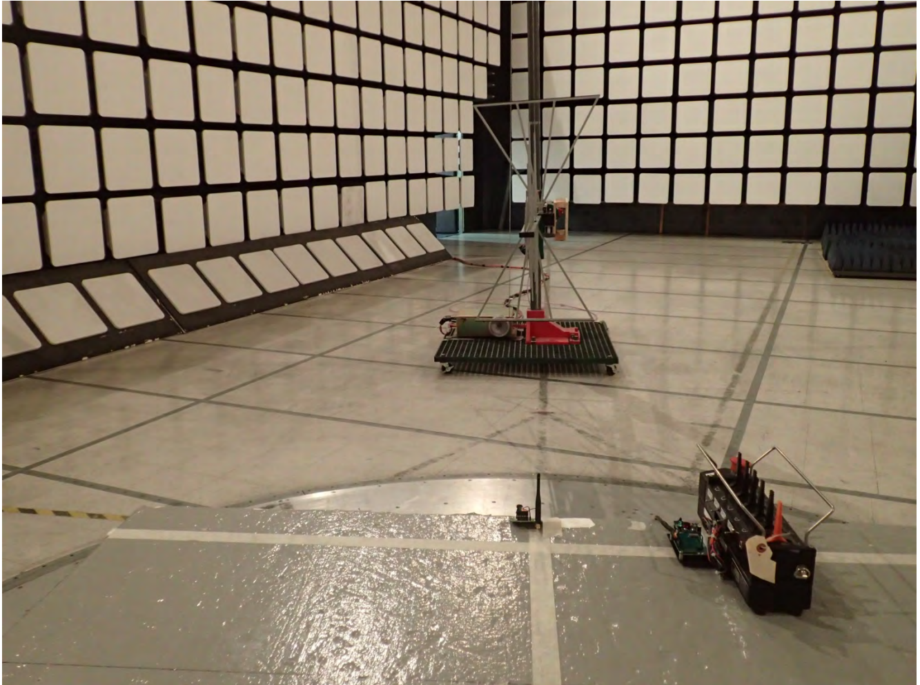
Radiated Emissions @ 3 m EUT with ANT-916-CW-RCL Antenna, Orthogonal Position 1
