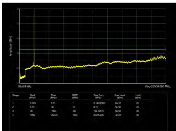
LTE Band 38 20MHz CH-Low 9kHz~26.5GHz
