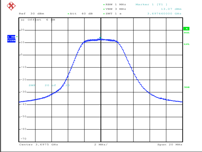
64QAM Middle channel
