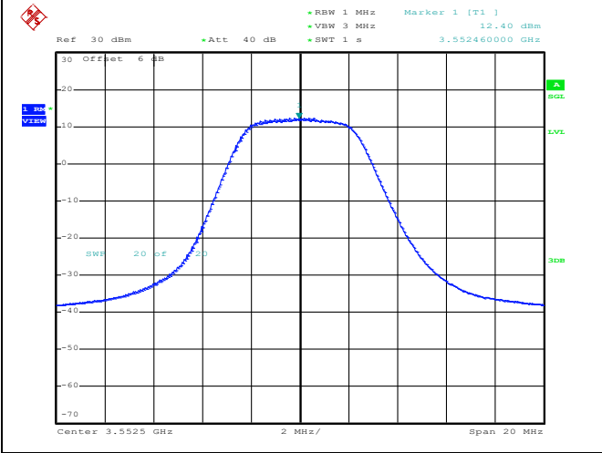
16QAM High channel
