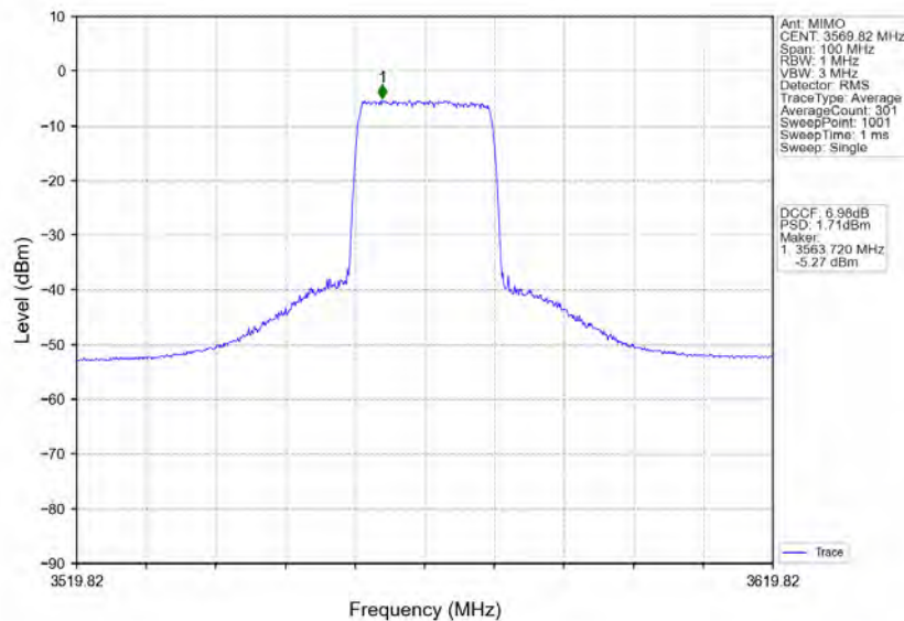
n48_30kHz_MIMO_NTNV_40MHz_CP-OFDM 64 QAM_3570MHz_Inner_Full
