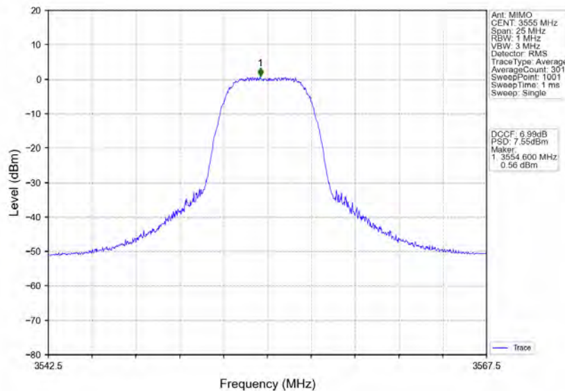
n48_30kHz_MIMO_NTNV_10MHz_CP-OFDM 64 QAM_3555MHz_Inner_Full
