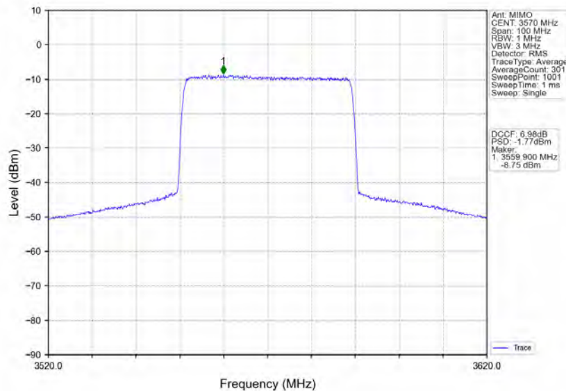
n48_30kHz_MIMO_NTNV_40MHz_CP-OFDM_16_QAM_3570MHz_Inner_Full
