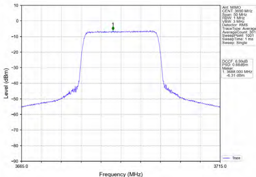
n48_30kHz_MIMO_NTNV_20MHz_CP-OFDM QPSK_3690MHz_Inner_Full
