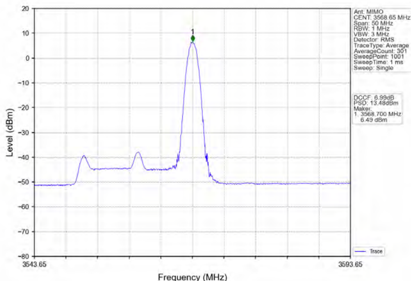
n48_30kHz_MIMO_NTNV_20MHz_CP-OFDM_16_QAM_3560.01MHz_Inner_1RB_Right
