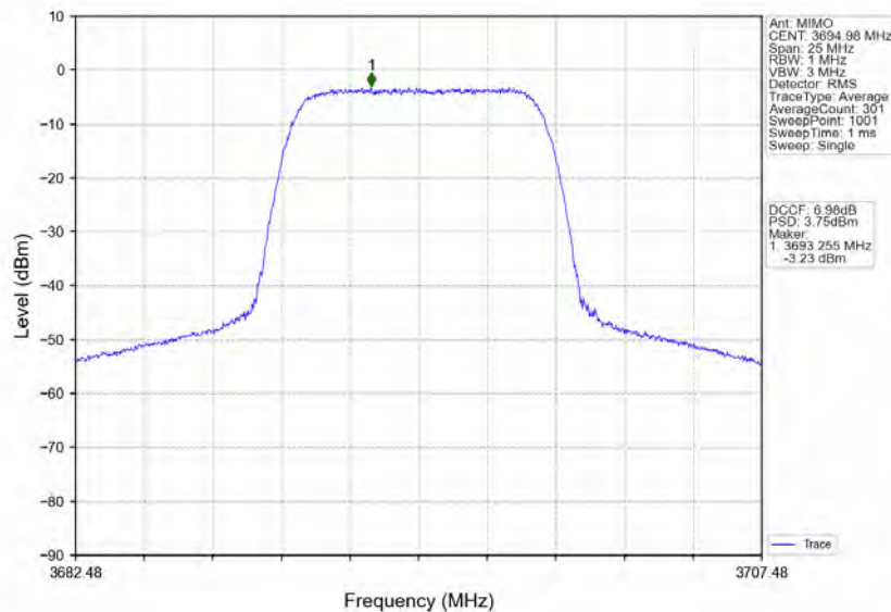
n48_30kHz_MIMO_NTNV_10MHz_CP-OFDM 16 QAM 3694.98MHz_Inner_Full
