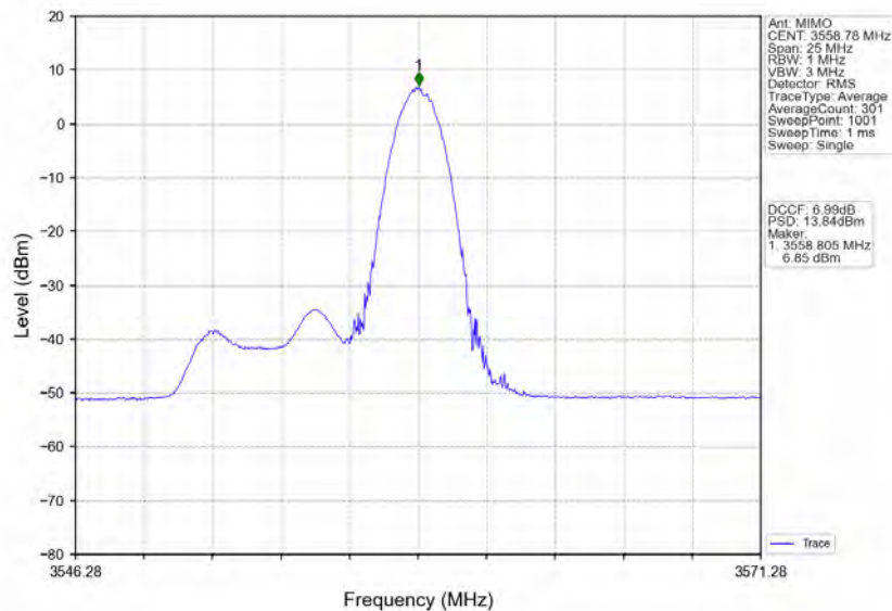
n48_30kHz_MIMO_NTNV_10MHz_CP-OFDM_256_QAM_3555MHz_Inner_1RB_Right
