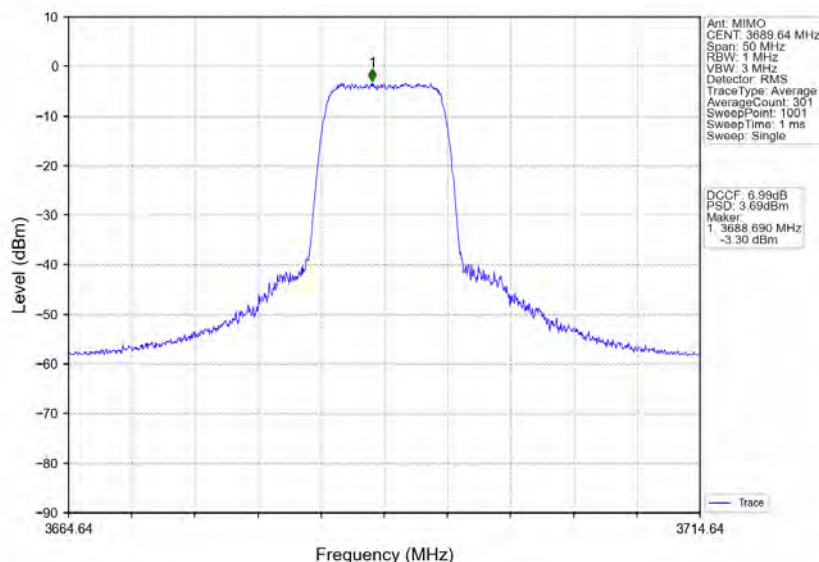
n48_30kHz_MIMO_NTNV_20MHz_CP-OFDM_64_QAM_3690MHz_Inner_Full
