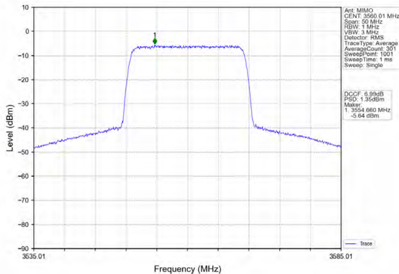
n48_30kHz_MIMO_NTNV_20MHz_CP-OFDM_16_QAM_3560.01MHz_Inner_Full
