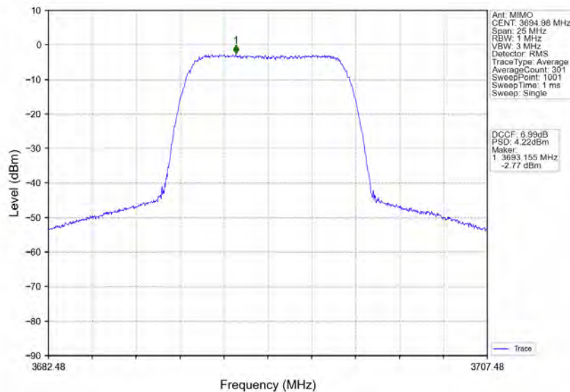
n48_30kHz_MIMO_NTNV_10MHz_CP-OFDM_256_QAM_3694.98MHz_Inner_Full
