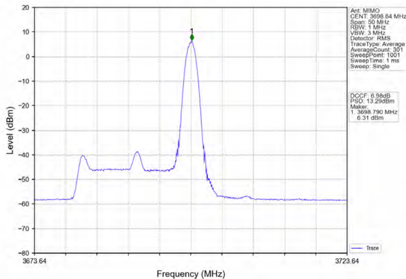
n48_30kHz_MIMO_NTNV_20MHz_CP-OFDM_16_QAM_3690MHz_Inner_1RB_Right
