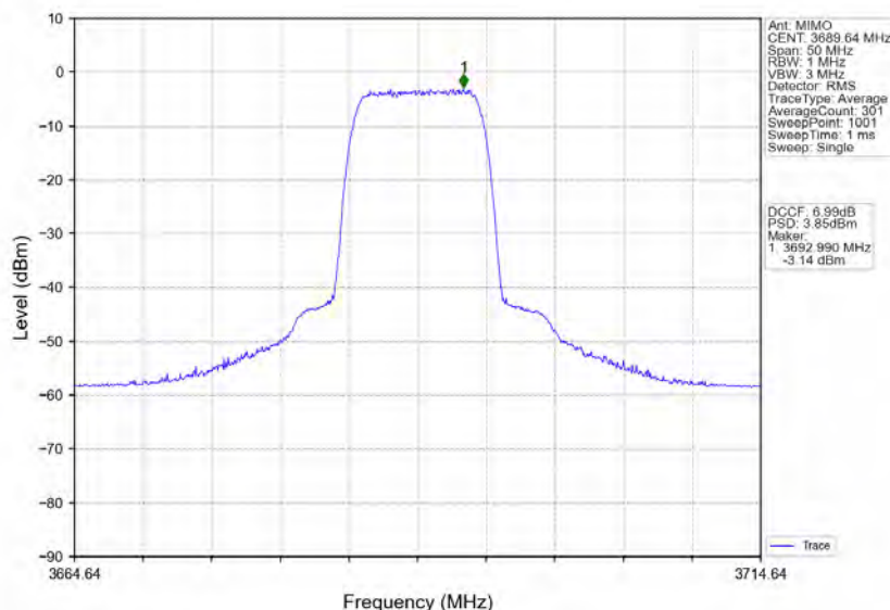
n48_30kHz_MIMO_NTNV_20MHz_CP-OFDM_256_QAM_3690MHz_Inner_Full
