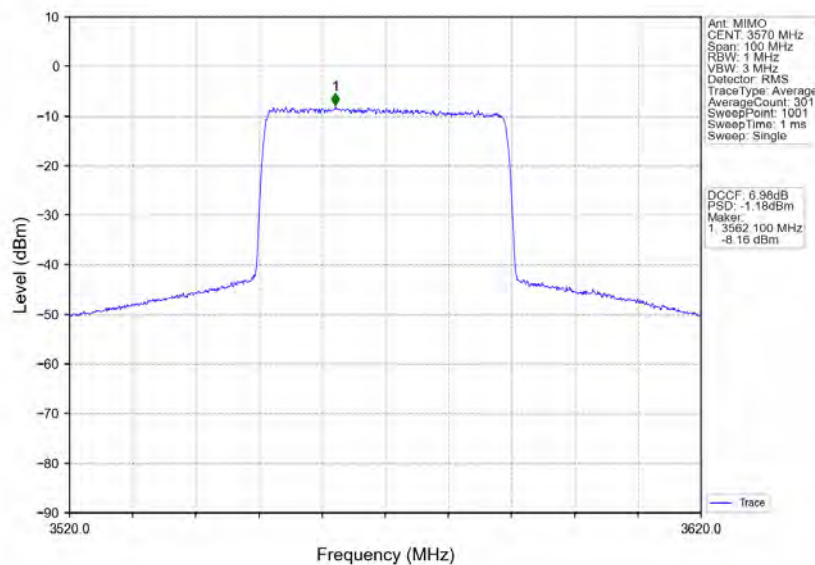
n48_30kHz_MIMO_NTNV_40MHz_CP-OFDM QPSK_3570MHz_Inner_Full
