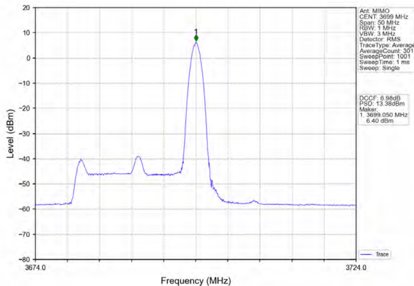
n48_30kHz_MIMO_NTNV_20MHz_CP-OFDM_16_QAM_3690MHz_Edge_1RB_Right
