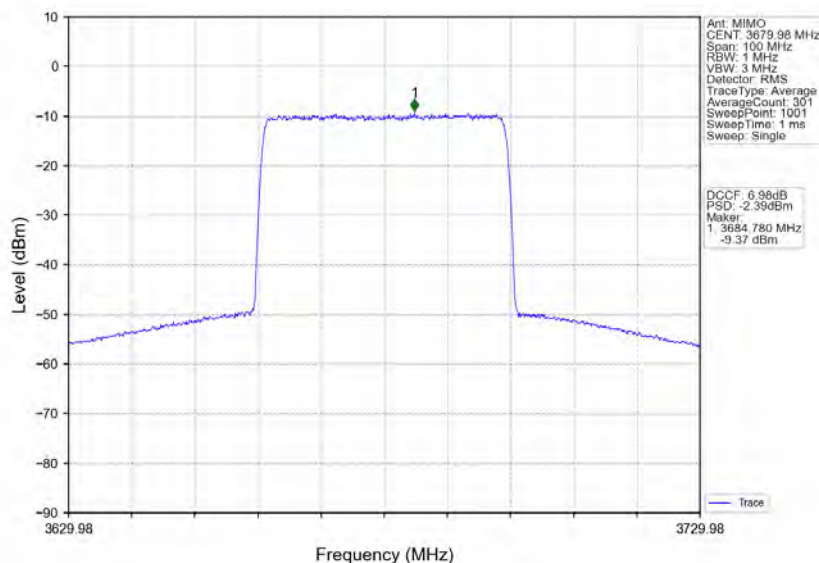
n48_30kHz_MIMO_NTNV_40MHz_CP-OFDM_256_QAM_3679.98MHz_Inner_Full
