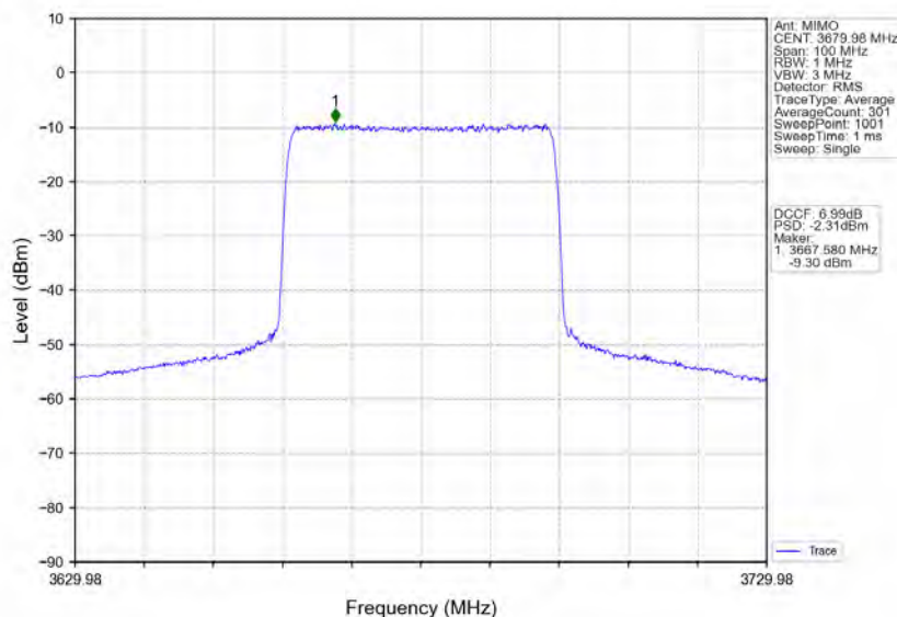
n48_30kHz_MIMO_NTNV_40MHz_CP-OFDM 16 QAM 3679.98MHz_Inner_Full
