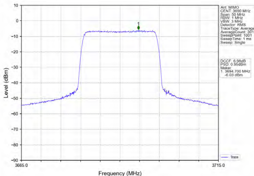
n48_30kHz_MIMO_NTNV_20MHz_CP-OFDM_64_QAM_3690MHz_Inner_Full
