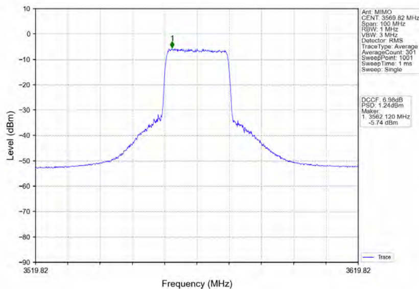
n48_30kHz_MIMO_NTNV_40MHz_CP-OFDM QPSK_3570MHz_Inner_Full
