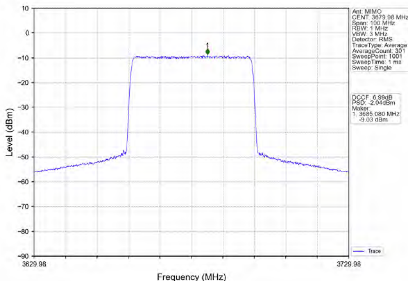
n48_30kHz_MIMO_NTNV_40MHz_CP-OFDM 64 QAM_3679.98MHz_Inner_Full
