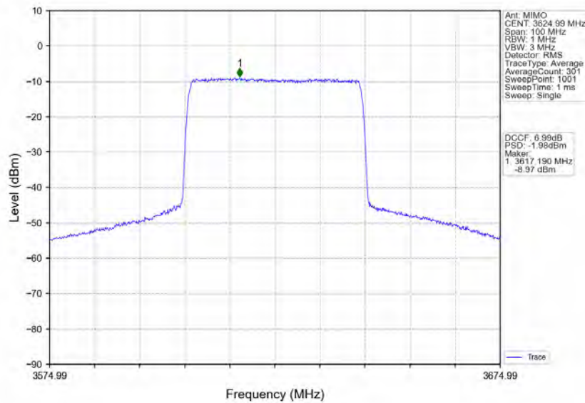
n48_30kHz_MIMO_NTNV_40MHz_CP-OFDM 64 QAM 3624.99MHz_Inner_Full
