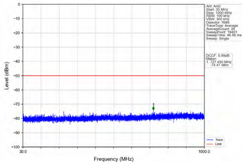
n48_30kHz_MIMO_NTNV_40MHz_CP-OFDM_QPSK_3570MHz_Outer_Full
