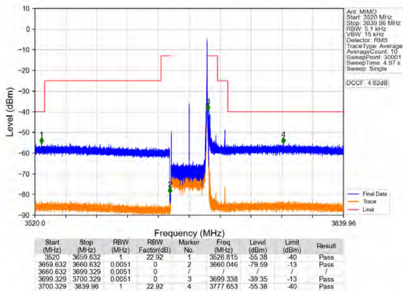
n48_30kHz_MIMO_NTNV_40MHz_CP-OFDM_QPSK_3679.98MHz_Inner_1RB_Right
