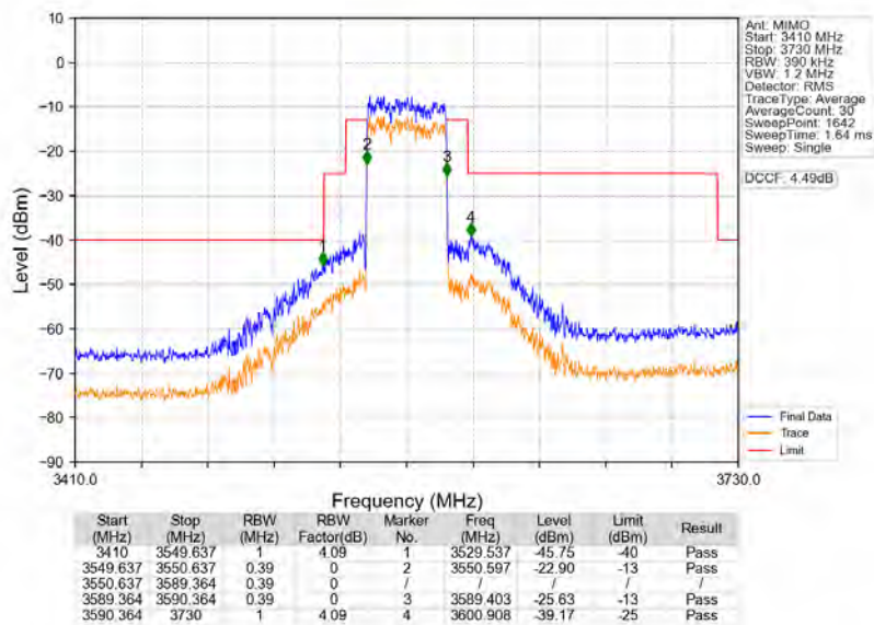
n48_30kHz_MIMO_NTNV_40MHz_CP-OFDM_QPSK_3570MHz_Outer_Full
