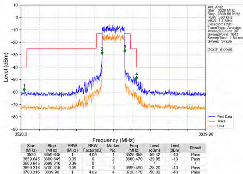
n48_30kHz_MIMO_NTNV_40MHz_CP-OFDM_QPSK_3679.98MHz_Outer_Full
