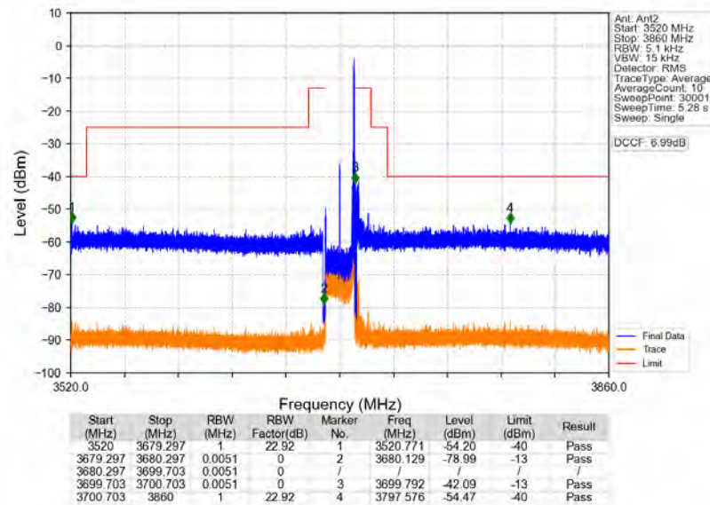
n78d_30kHz_MIMO_NTNV_20MHz_CP-OFDM_QPSK_3690MHz_Edge_1RB_Right
