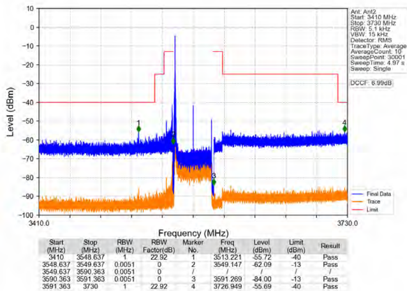
n78d_30kHz_MIMO_NTNV_40MHz_CP-OFDM_QPSK_3570MHz_Edge_1RB_Left
