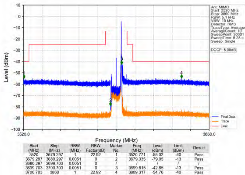
n78d_30kHz_MIMO_NTNV_20MHz_CP-OFDM_QPSK_3690MHz_Edge_1RB_Right
