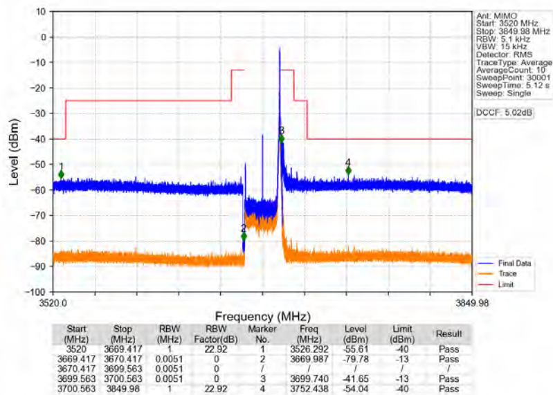
n78d_30kHz_MIMO_NTNV_30MHz_CP-OFDM_QPSK_3684.99MHz_Inner_1RB_Right
