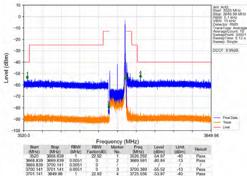
n78d_30kHz_MIMO_NTNV_30MHz_CP-OFDM_QPSK_3684.99MHz_Inner_1RB_Right
