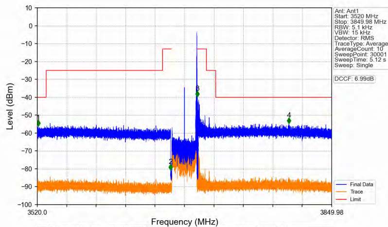
n78d_30kHz_MIMO_NTNV_30MHz_CP-OFDM_QPSK_3684.99MHz_Edge_1RB_Right
