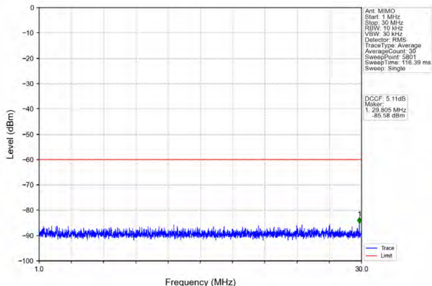
n78d_30kHz_MIMO_NTNV_20MHz_CP-OFDM_QPSK_3690MHz_Inner_1RB_Right
