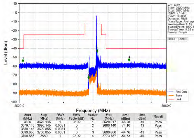
n78d_30kHz_MIMO_NTNV_20MHz_CP-OFDM_QPSK_3690MHz_Inner_1RB_Right
