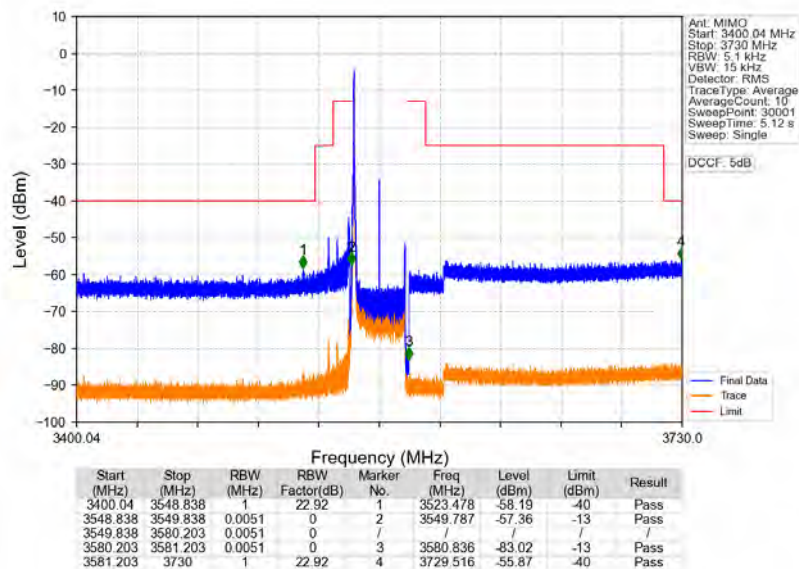
n78d_30kHz_MIMO_NTNV_30MHz_CP-OFDM_QPSK_3565.02MHz_Edge_1RB_Left
