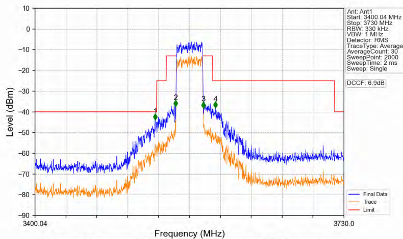
n78d_30kHz_MIMO_NTNV_30MHz_CP-OFDM_QPSK_3565.02MHz_Outer_Full
