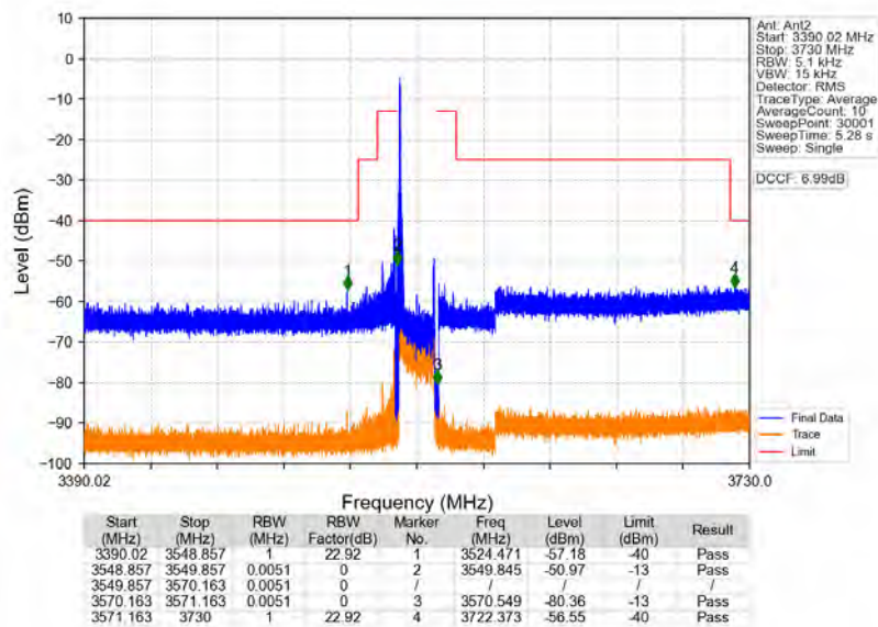
n78d_30kHz_MIMO_NTNV_20MHz_CP-OFDM_QPSK_3560.01MHz_Inner_1RB_Left
