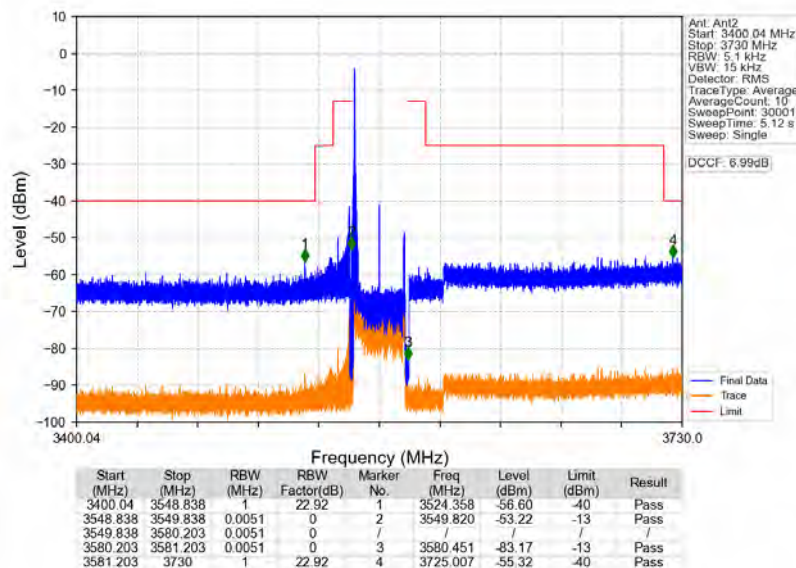
n78d_30kHz_MIMO_NTNV_30MHz_CP-OFDM_QPSK_3565.02MHz_Inner_1RB_Left
