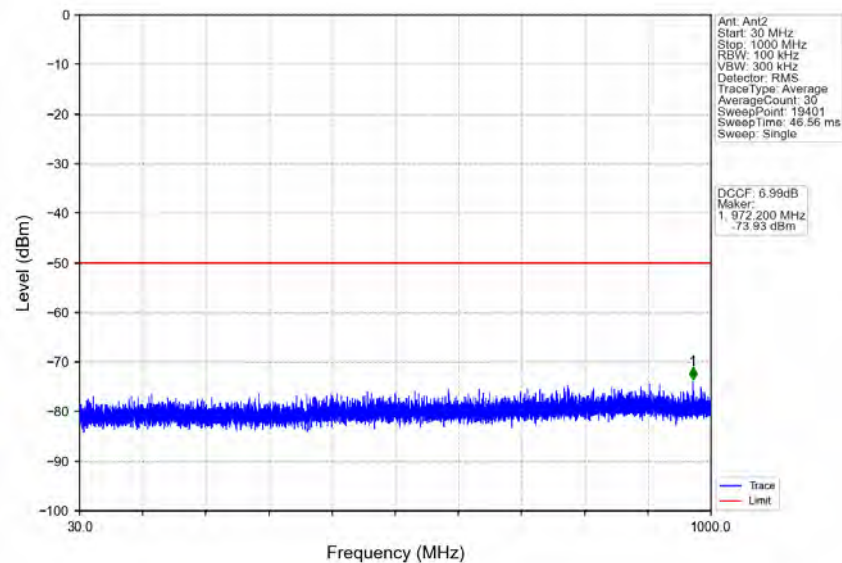
n78d_30kHz_MIMO_NTNV_20MHz_CP-OFDM_QPSK_3690MHz_Outer_Full
