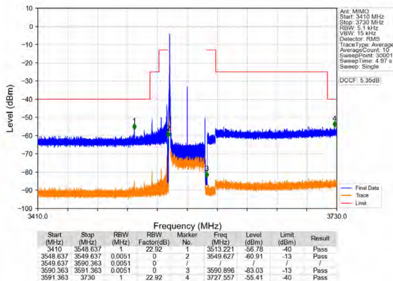
n78d_30kHz_MIMO_NTNV_40MHz_CP-OFDM_QPSK_3570MHz_Edge_1RB_Left
