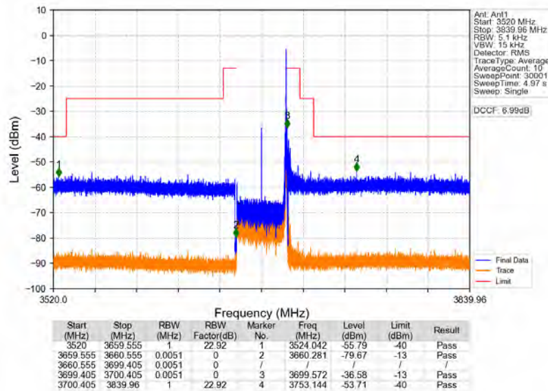
n78d_30kHz_MIMO_NTNV_40MHz_CP-OFDM QPSK_3679.98MHz_Edge_1RB_Right
