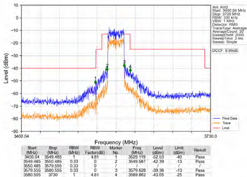
n78d_30kHz_MIMO_NTNV_30MHz_CP-OFDM_QPSK_3565.02MHz_Outer_Full
