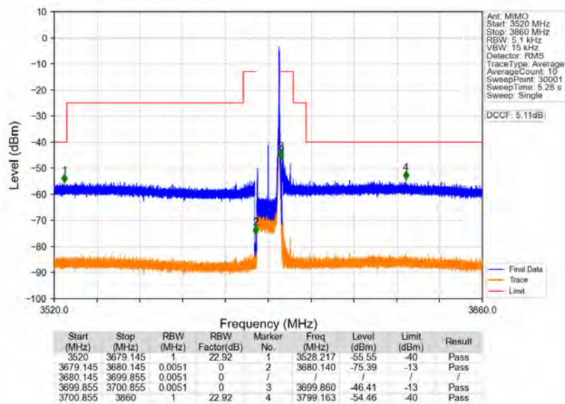
n78d_30kHz_MIMO_NTNV_20MHz_CP-OFDM_QPSK_3690MHz_Inner_1RB_Right
