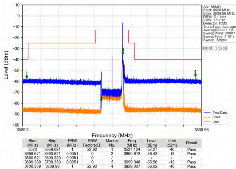
n78d_30kHz_MIMO_NTNV_40MHz_CP-OFDM_QPSK_3679.98MHz_Edge_1RB_Right
