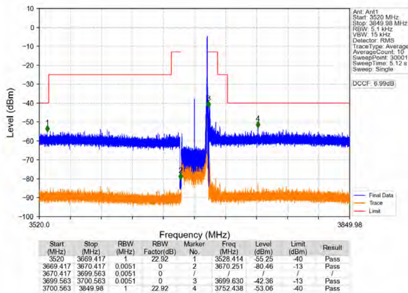
n78d_30kHz_MIMO_NTNV_30MHz_CP-OFDM QPSK_3684.99MHz_Inner_1RB_Right
