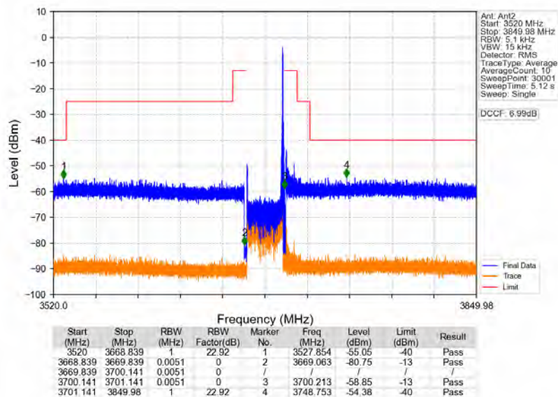
n78d_30kHz_MIMO_NTNV_30MHz_CP-OFDM_QPSK_3684.99MHz_Edge_1RB_Right
