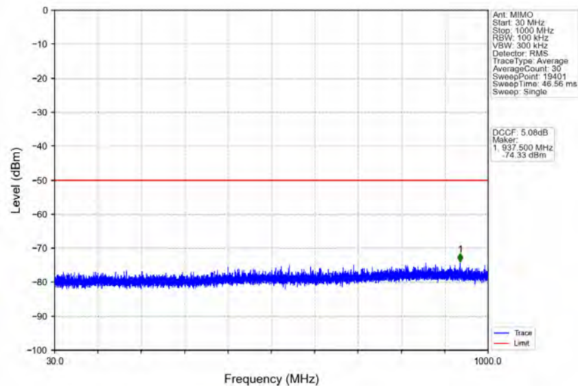
n78d_30kHz_MIMO_NTNV_20MHz_CP-OFDM QPSK_3690MHz_Edge_1RB_Right
