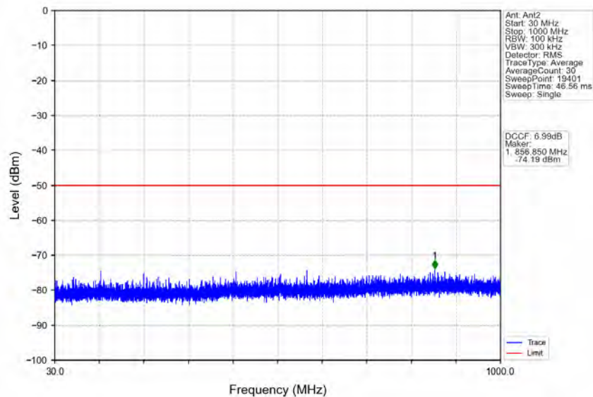
n78d_30kHz_MIMO_NTNV_40MHz_CP-OFDM_QPSK_3570MHz_Inner_1RB_Left
