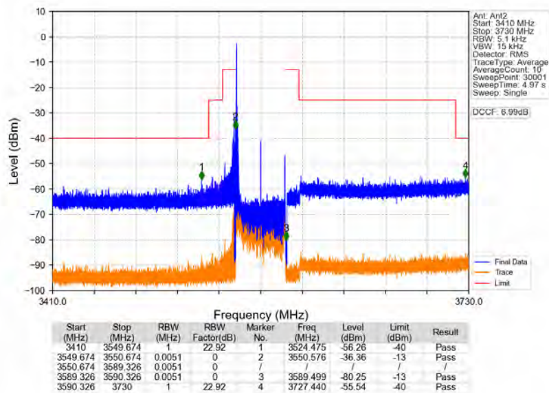
n78d_30kHz_MIMO_NTNV_40MHz_CP-OFDM_QPSK_3570MHz_Inner_1RB_Left
