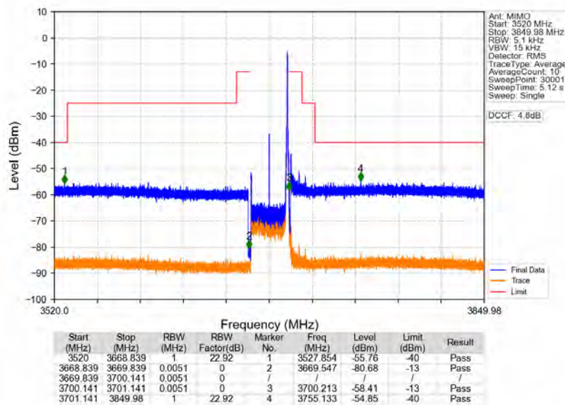
n78d_30kHz_MIMO_NTNV_30MHz_CP-OFDM_QPSK_3684.99MHz_Edge_1RB_Right
