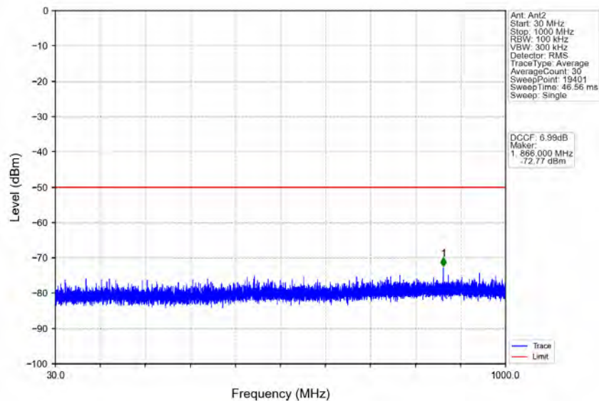
n78d_30kHz_MIMO_NTNV_30MHz_CP-OFDM_QPSK_3565.02MHz_Edge_1RB_Left
