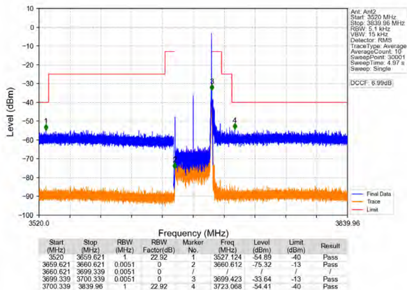
n78d_30kHz_MIMO_NTNV_40MHz_CP-OFDM_QPSK_3679.98MHz_Edge_1RB_Right
