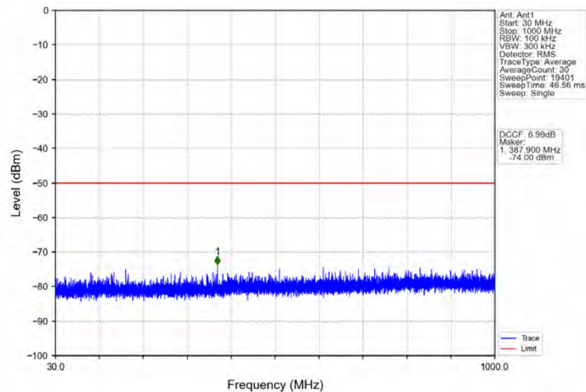
n78d_30kHz_MIMO_NTNV_30MHz_CP-OFDM_QPSK_3684.99MHz_Inner_1RB_Right
