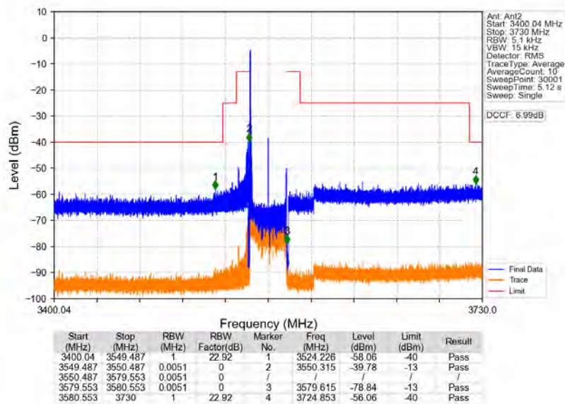
n78d_30kHz_MIMO_NTNV_30MHz_CP-OFDM_QPSK_3565.02MHz_Edge_1RB_Left
