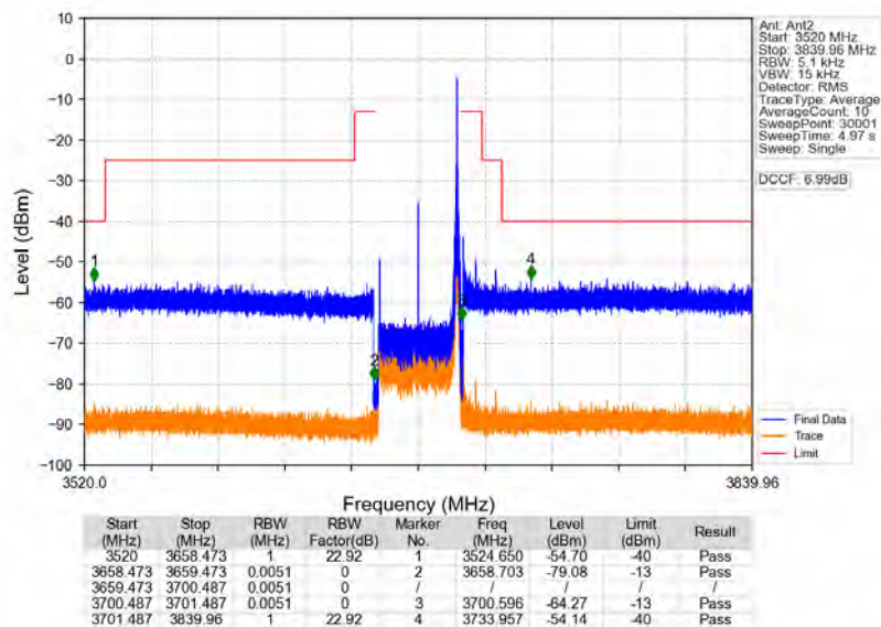
n78d_30kHz_MIMO_NTNV_40MHz_CP-OFDM_QPSK_3679.98MHz_Inner_1RB_Right
