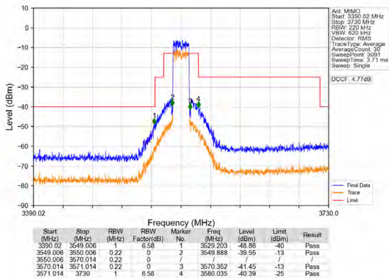
n78d_30kHz_MIMO_NTNV_20MHz_CP-OFDM_QPSK_3560.01MHz_Outer_Full
