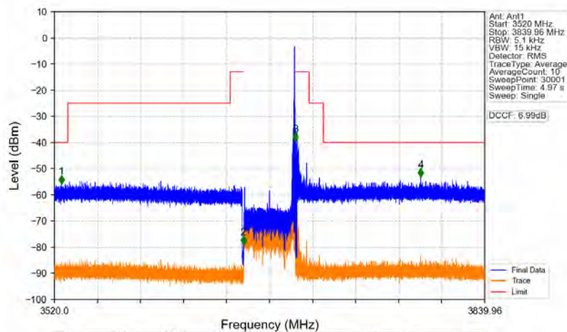
n78d_30kHz_MIMO_NTNV_40MHz_CP-OFDM_QPSK_3679.98MHz_Inner_1RB_Right
