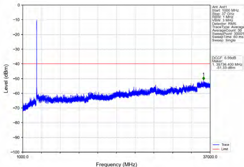
n78d_30kHz_MIMO_NTNV_40MHz_CP-OFDM_QPSK_3679.98MHz_Outer_Full
