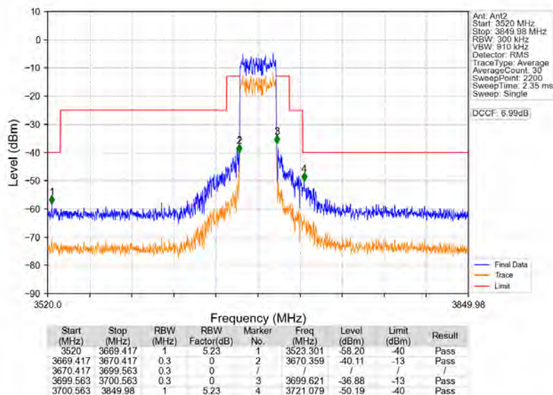
n78d_30kHz_MIMO_NTNV_30MHz_CP-OFDM_QPSK_3684.99MHz_Outer_Full
