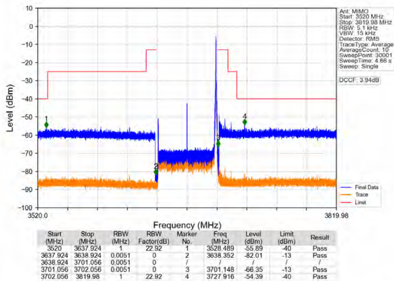
n78d_30kHz_MIMO_NTNV_60MHz_CP-OFDM_QPSK_3669.99MHz_Edge_1RB_Right
