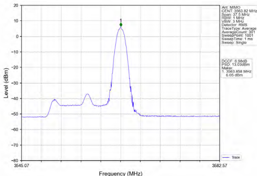
n78d_30kHz_MIMO_NTNV_15MHz_CP-OFDM_16_QAM_3557.52MHz_Inner_1RB_Right
