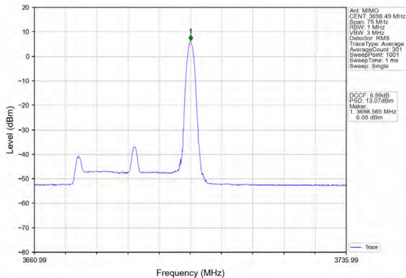
n78d_30kHz_MIMO_NTNV_30MHz_CP-OFDM 64 QAM_3684.99MHz_Inner_1RB_Right
