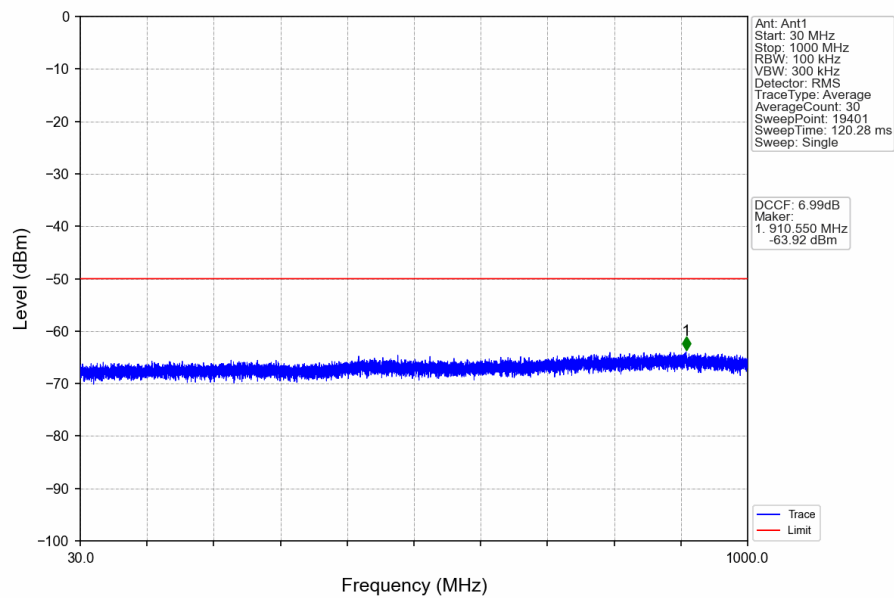
n78d_30kHz_SISO_NTNV_40MHz_CP-OFDM_QPSK_3624.99MHz_Edge_1RB_Left
