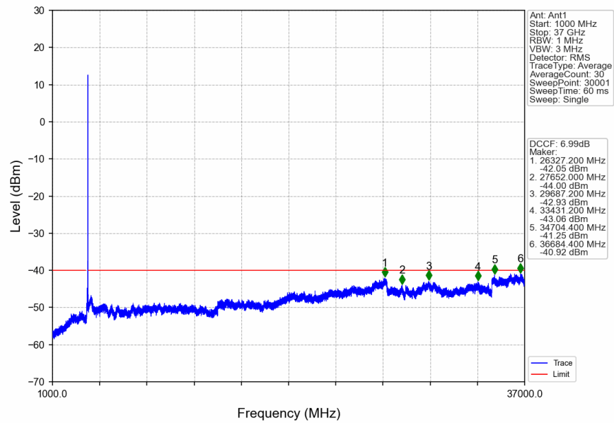
n78d_30kHz_SISO_NTNV_50MHz_DFT-s-OFDM QPSK_3675MHz_Edge_1RB_Right
