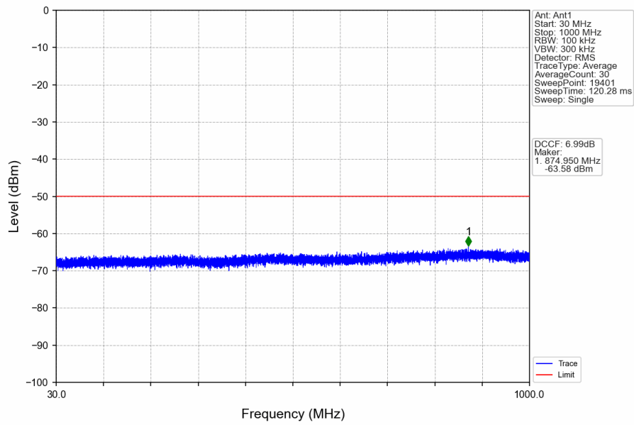
n78d_30kHz_SISO_NTNV_50MHz_DFT-s-OFDM QPSK_3675MHz_Edge_1RB_Right
