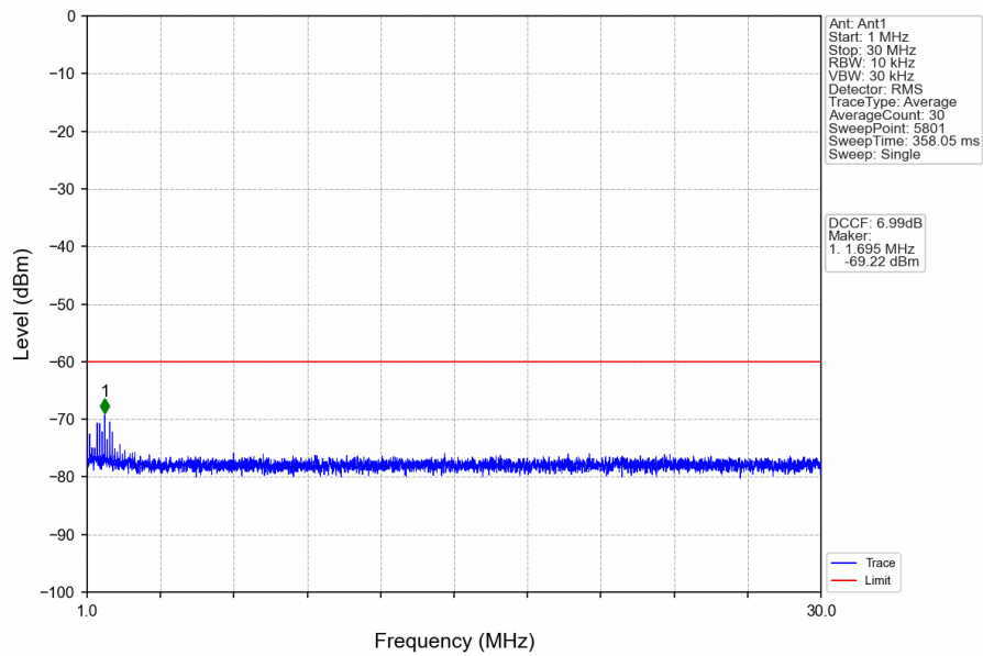
n78d_30kHz_SISO_NTNV_50MHz_CP-OFDM_QPSK_3575.01MHz_Edge_1RB_Left
