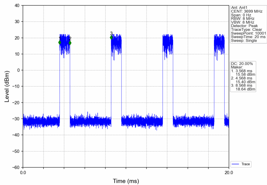
n78d_30kHz_SISO_NTNV_20MHz_CP-OFDM_16_QAM_3690MHz_Edge_1RB_Right
