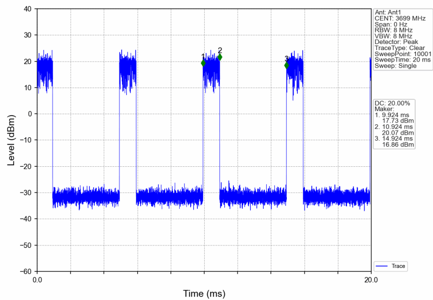
n78d_30kHz_SISO_NTNV_20MHz_CP-OFDM_64_QAM_3690MHz_Edge_1RB_Right
